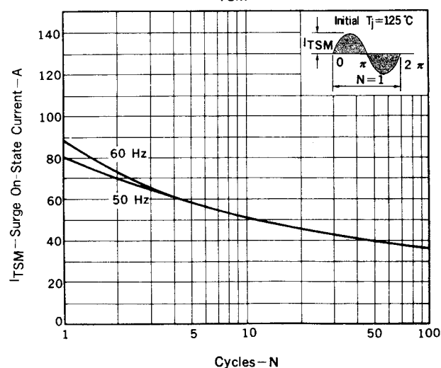
Fig. 2 I_{\text{TSM}} RATING
