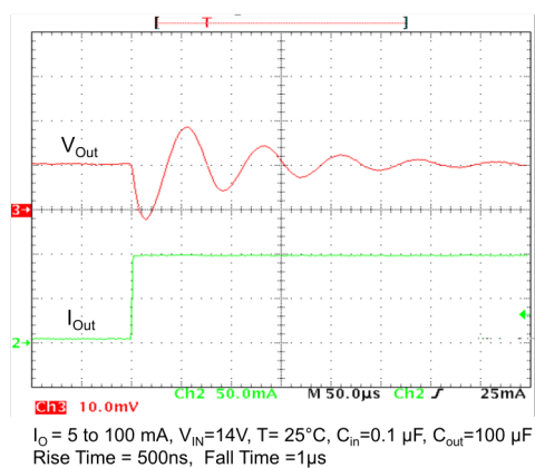
Figure 24. Load transient
