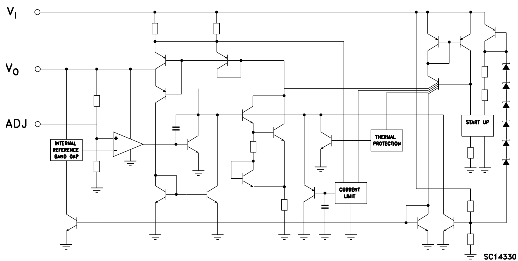
Figure 2. Schematic diagram
