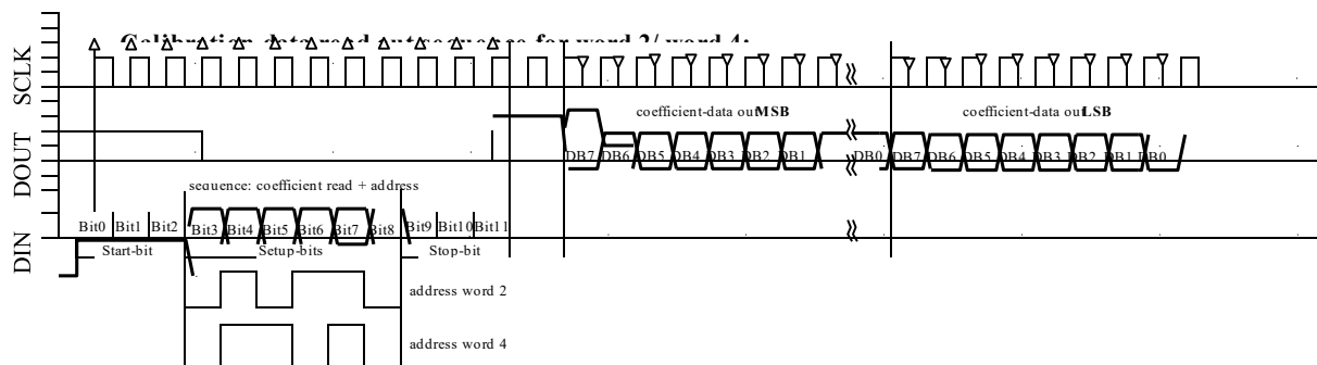
Fig. 6d: W2, W4 READING sequence
