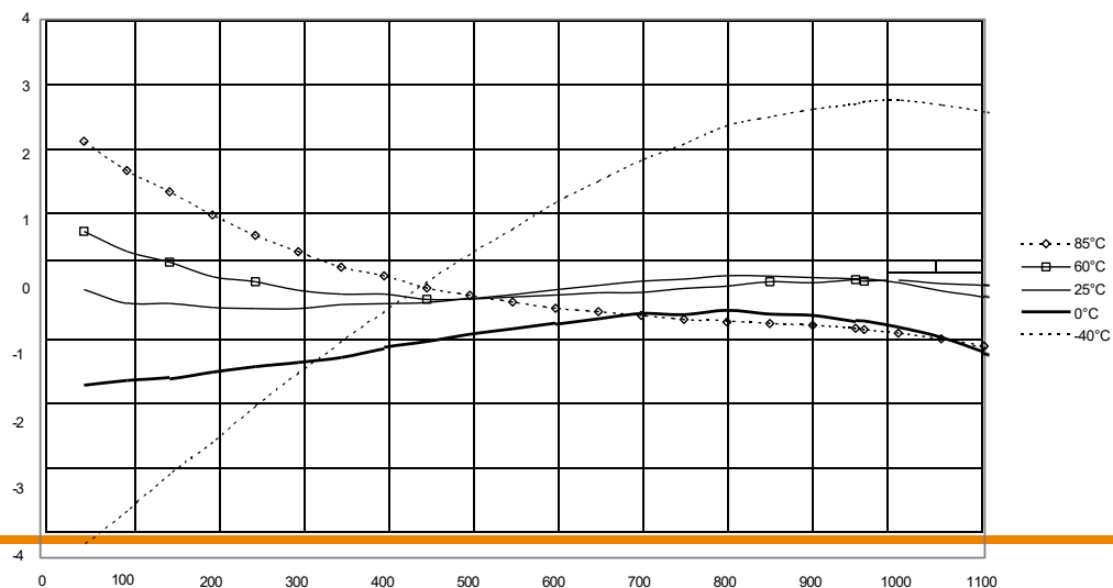
Absolute Pressure Accuracy after Calibration, 2nd order compensation
