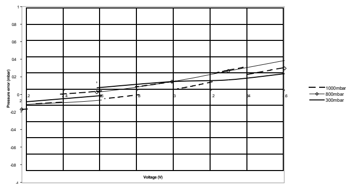
Pressure error vs supply voltage (typical)
