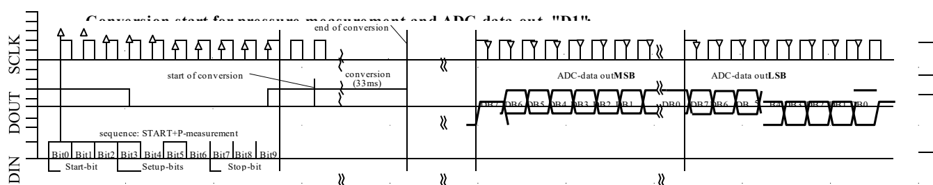
Fig. 6a: D1 ACQUISITION sequence
