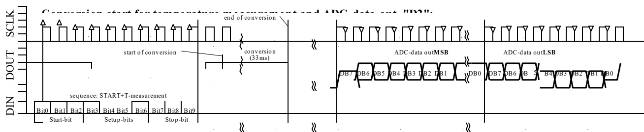
Fig. 6b: D2 ACQUISITION sequence
