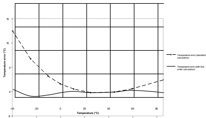
Temperature Error Accuracy vs temperature (typical)
