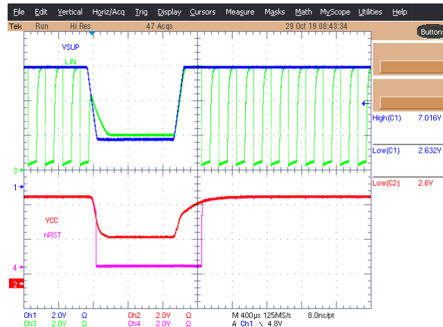
Figure 10-10. TLIN1028S-Q1 Brownout
