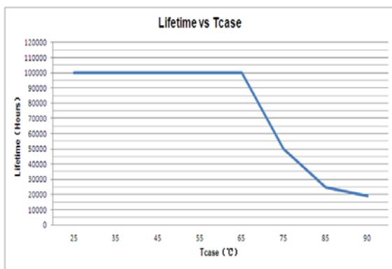
LIFETIME Curve
