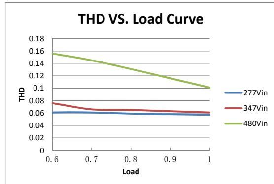
THD Curve
