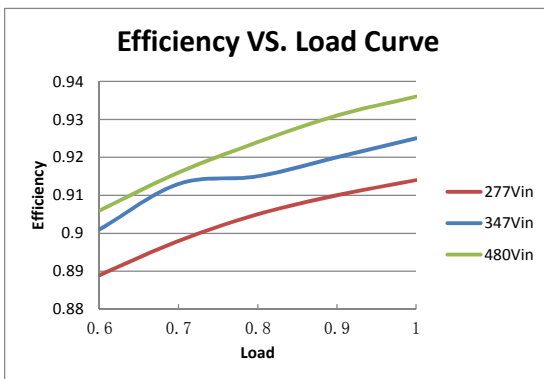
eff Curve
