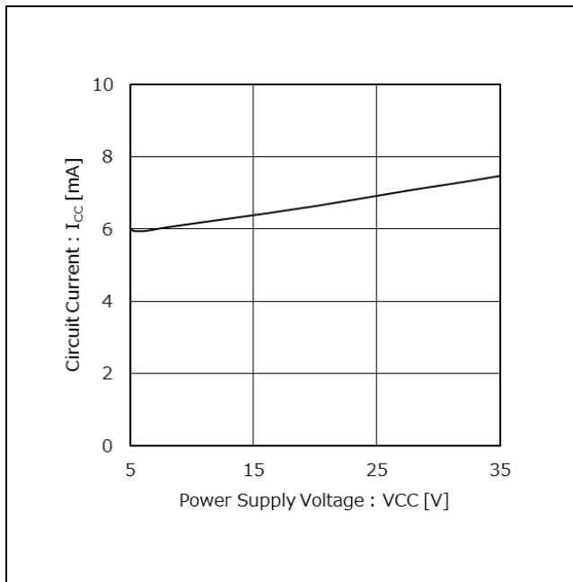
Figure 8. Circuit Current vs Power Supply Voltage ( V_{CC} = 4.5\text{ V} to 35\text{ V} , V_{EN} = 3.3\text{ V} , V_{PWM} = 0\text{ V} )
