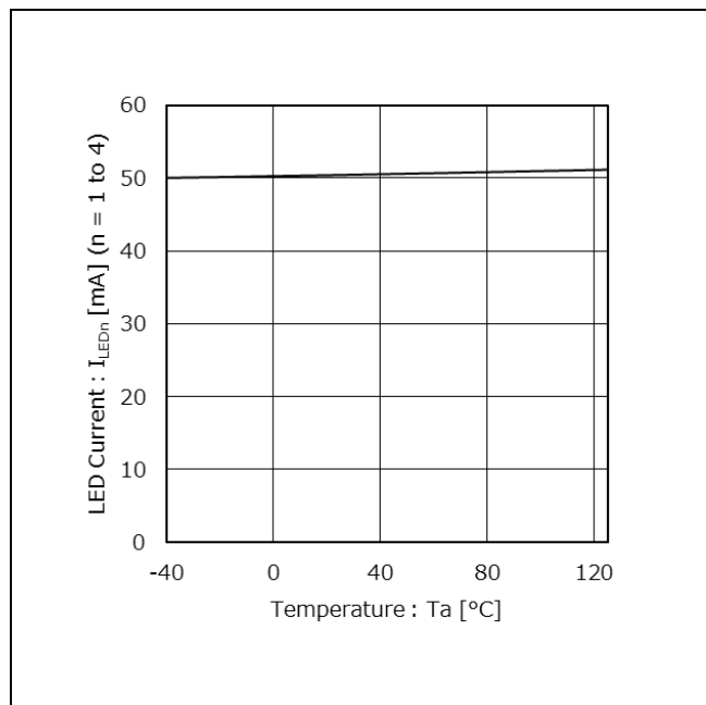
Figure 13. LED Current vs Temperature ( V_{CC} = 12\text{ V} , V_{EN} = 3.3\text{ V} , V_{LEDn} = 2\text{ V} (n = 1 to 4), V_{PWM} = V_{VREG} )
