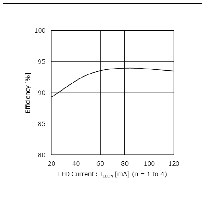
Figure 15. Efficiency vs LED Current(n = 1 to 4) (Boost Application) ( T_a = 25\text{ }^{\circ}\text{C} , V_{CC} = 12\text{ V} , V_{EN} = 3.3\text{ V} , V_{PWM} = V_{VREG} , 8 LED loads per channel, all channels have loads)
