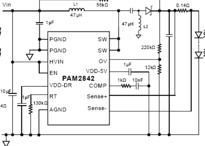
Buck/Boost (Sepic) with High Side Current Sense
