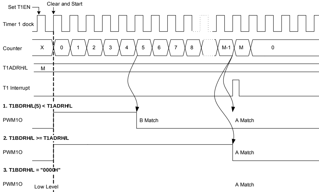
Figure 11.20 16-Bit PPG Mode Timming chart for Timer 1
