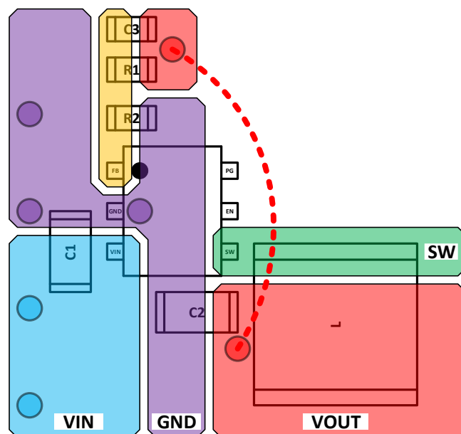
Figure 43. Recommended AP61302 PCB Layout
