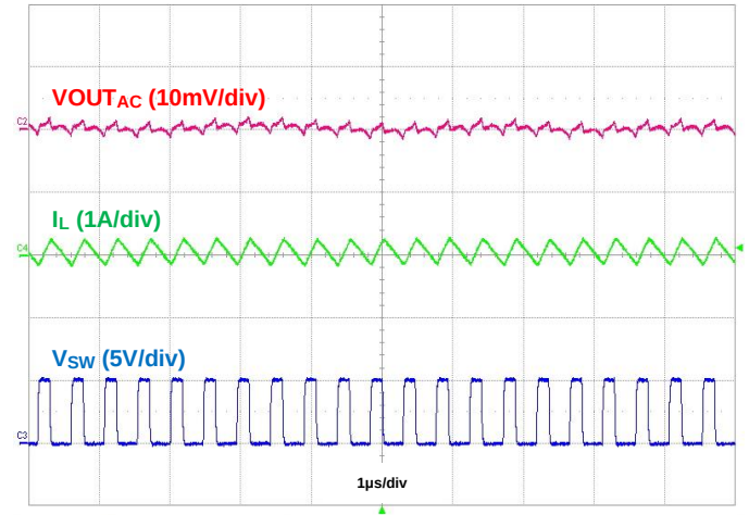
Figure 28. Output Voltage Ripple, IOU = 50mA
