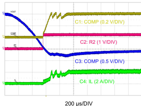
Figure 9-4. Automatic Wake-Up
