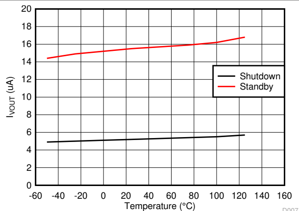
Figure 7-7. I_{VOUT} vs Temperature
