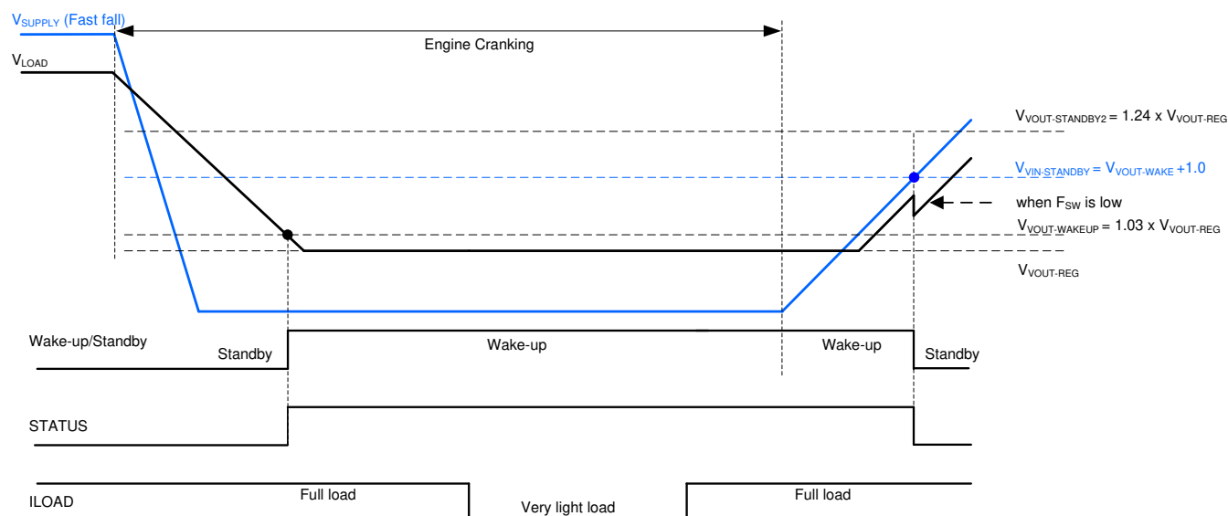
Figure 8-4. Automatic Wake-Up and Standby Operation in the SS Configuration (With Fast V_{SUPPLY} Fall and Slow Switching)
