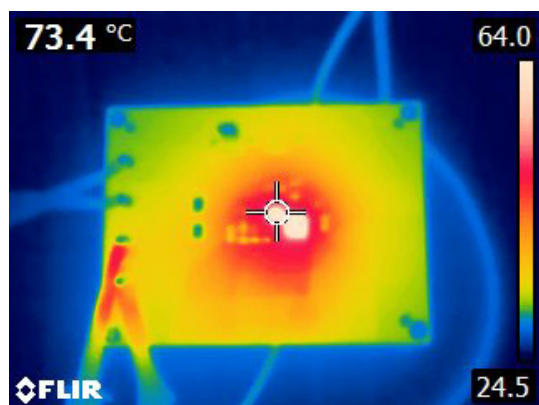
Figure 21. Thermal Image, 24V IN , 3.3V OUT , 400kHz, 5A, QFN, T_J = 73.4^{\circ}\text{C}
