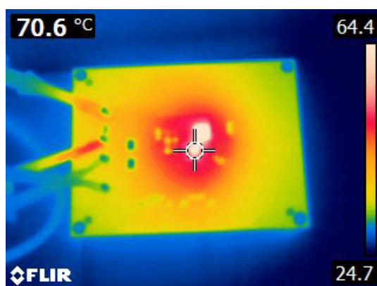
Figure 23. Thermal Image, 24V IN , 3.3V OUT , 400kHz, 5A, HTSSOP, T_J = 70.6^{\circ}\text{C}
