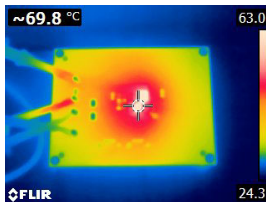
Figure 22. Thermal Image, 12V IN , 3.3V OUT , 400kHz, 5A, HTSSOP, T_J = 69.8^{\circ}\text{C}
