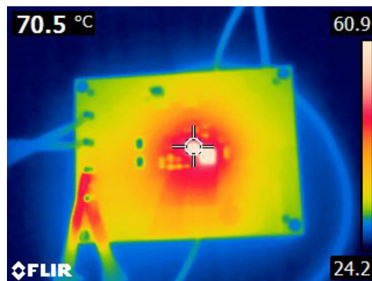
Figure 20. Thermal Image, 12V IN , 3.3V OUT , 400kHz, 5A, QFN, T_J = 70.5^{\circ}\text{C}
