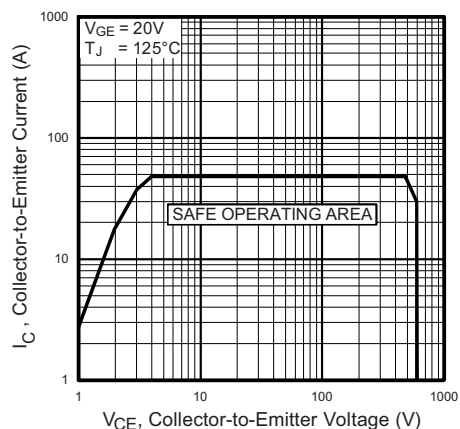
Fig. 12 - Turn-Off SOA
