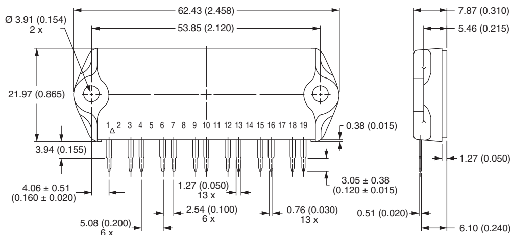
IMS-2 Package Outline (13 Pins)
