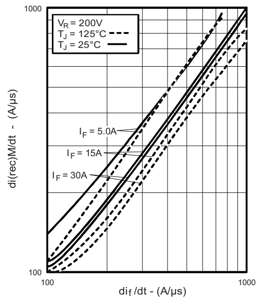
Fig. 17 - Typical dl_{(rec)M}/dt vs di_F/dt
