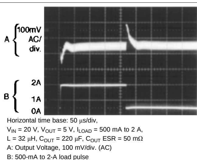
Figure 42. Load Transient Response for Continuous Mode
