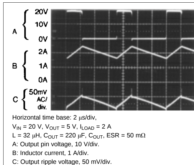
Figure 41. Continuous Mode Switching Waveforms
