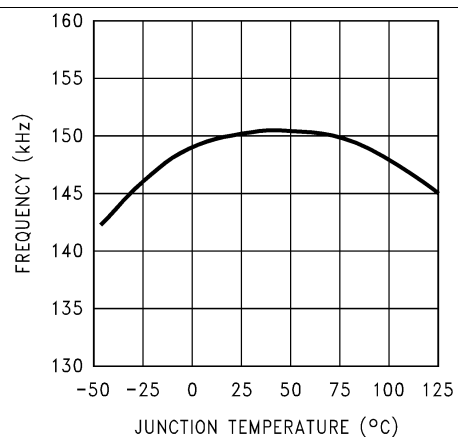
Figure 12. Switching Frequency
