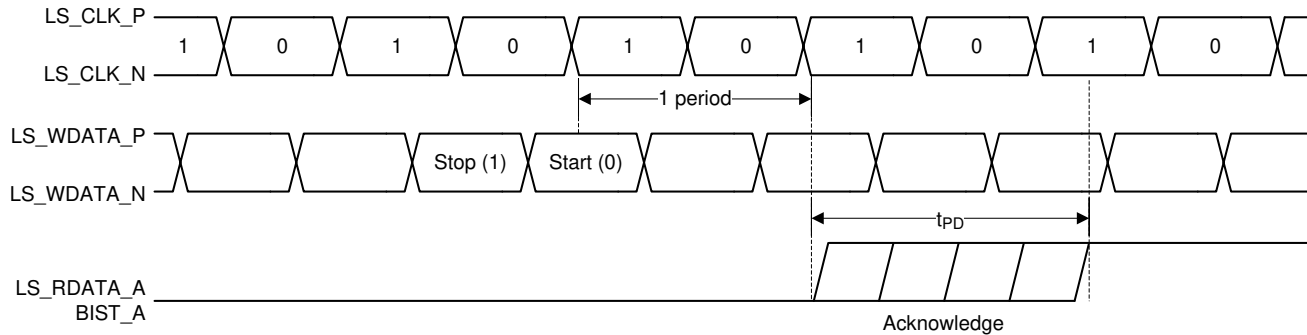
Figure 5-2. Switching Characteristics
