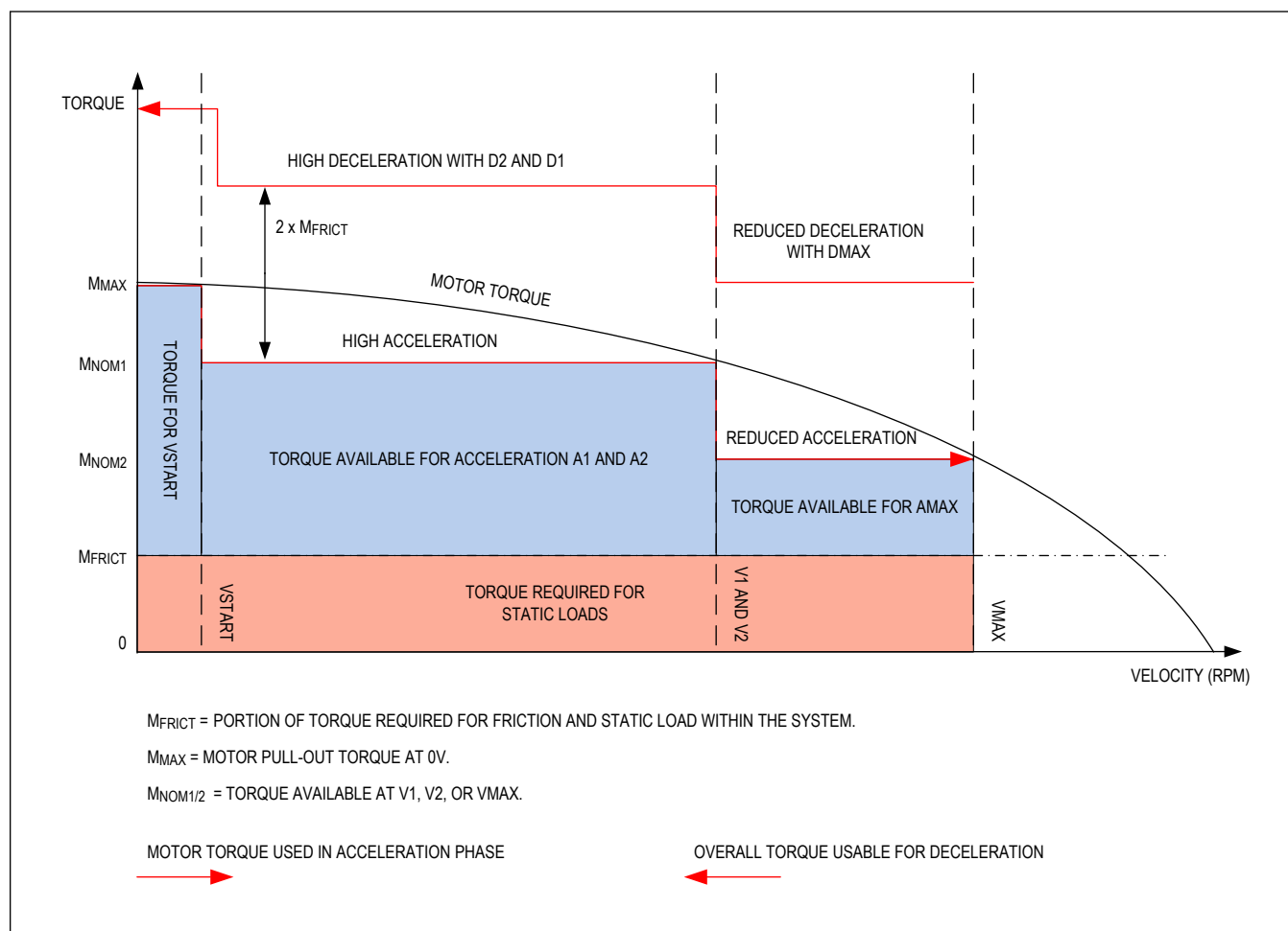
Figure 26. Optimized Motor Torque Usage with the Ramp Generator
