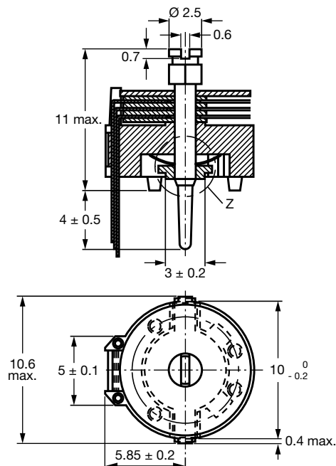
ROUND HEAD
