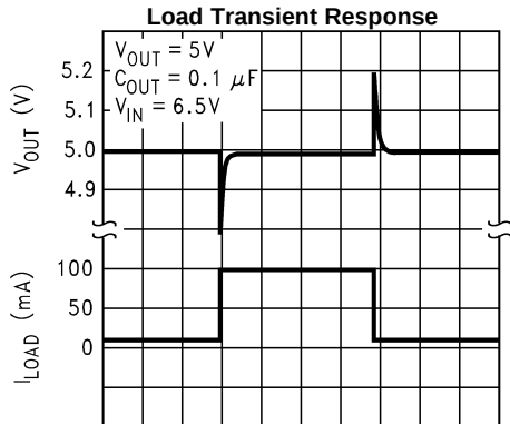
50 \mu s /Div Figure 14.
