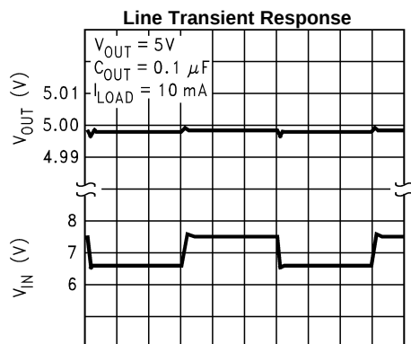
200 \mu s /Div Figure 10.
