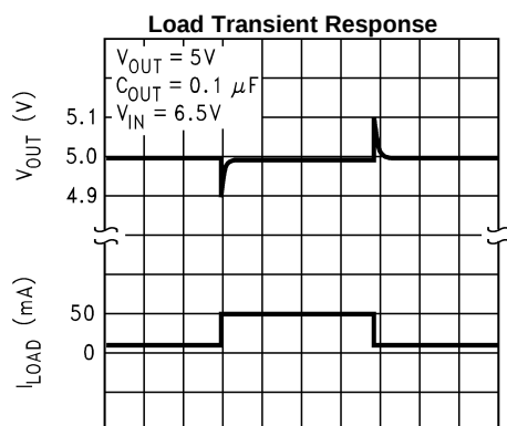
50 \mu s /Div Figure 12.
