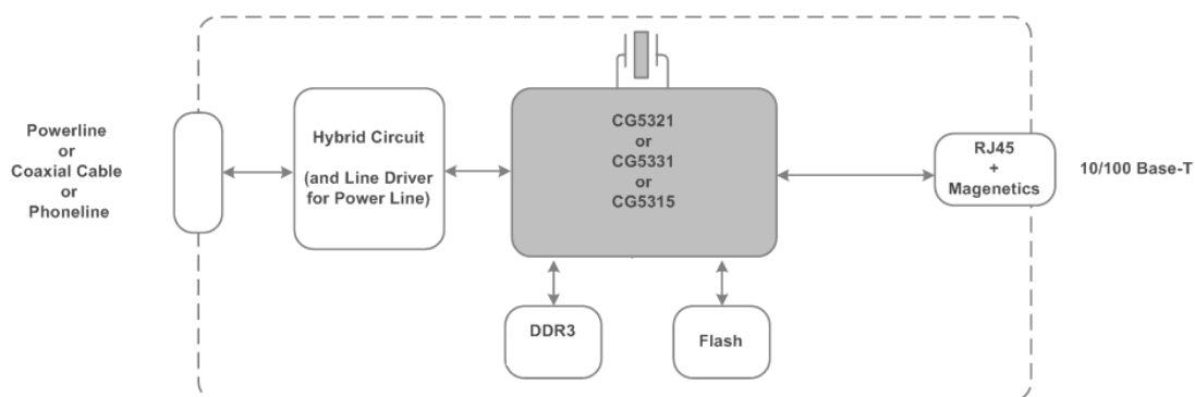
Figure 1: G.hn to Ethernet Bridges
