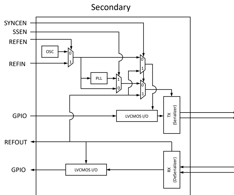
Figure 3 Clock Tree diagram of Secondary chip
