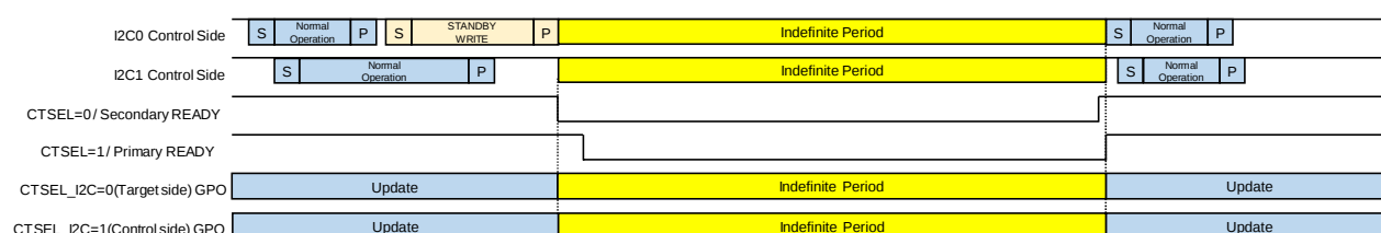
Figure 31 Standby => Normal (CTSEL_I2C=0/Secondary , CTSEL_I2C=1/Primary)
