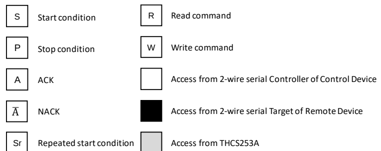
Figure 12 2-wire serial target register access
