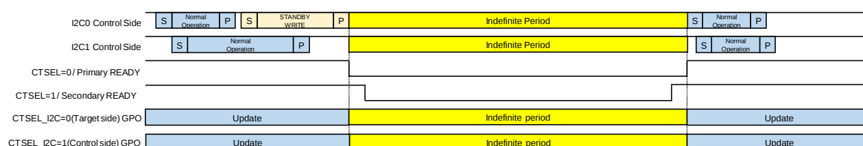
Figure 30 Standby => Normal (CTSEL_I2C=0/Primary , CTSEL_I2C=1/Secondary)
