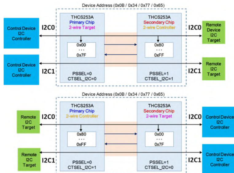
Figure 9 2-wire serial interface accessible range
