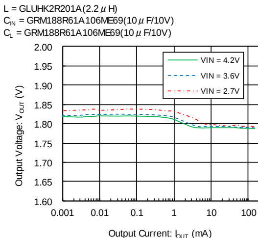
XC9276( V_{OUT}=1.8V )
