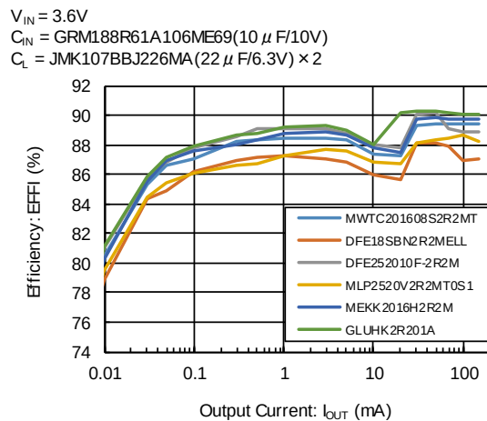
XC9276( V_{OUT}=1.8V )
