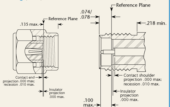
Jack (female)
