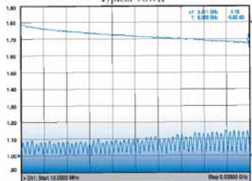
Typical VSWR
