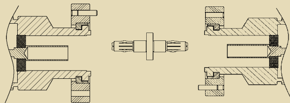
Jack (female)
