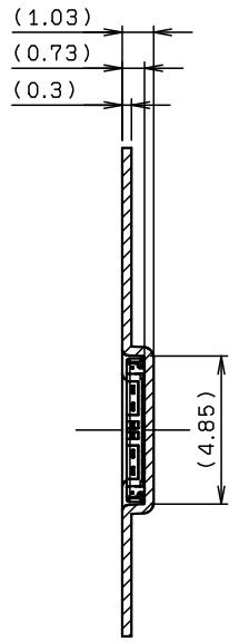
SECT. E-E
