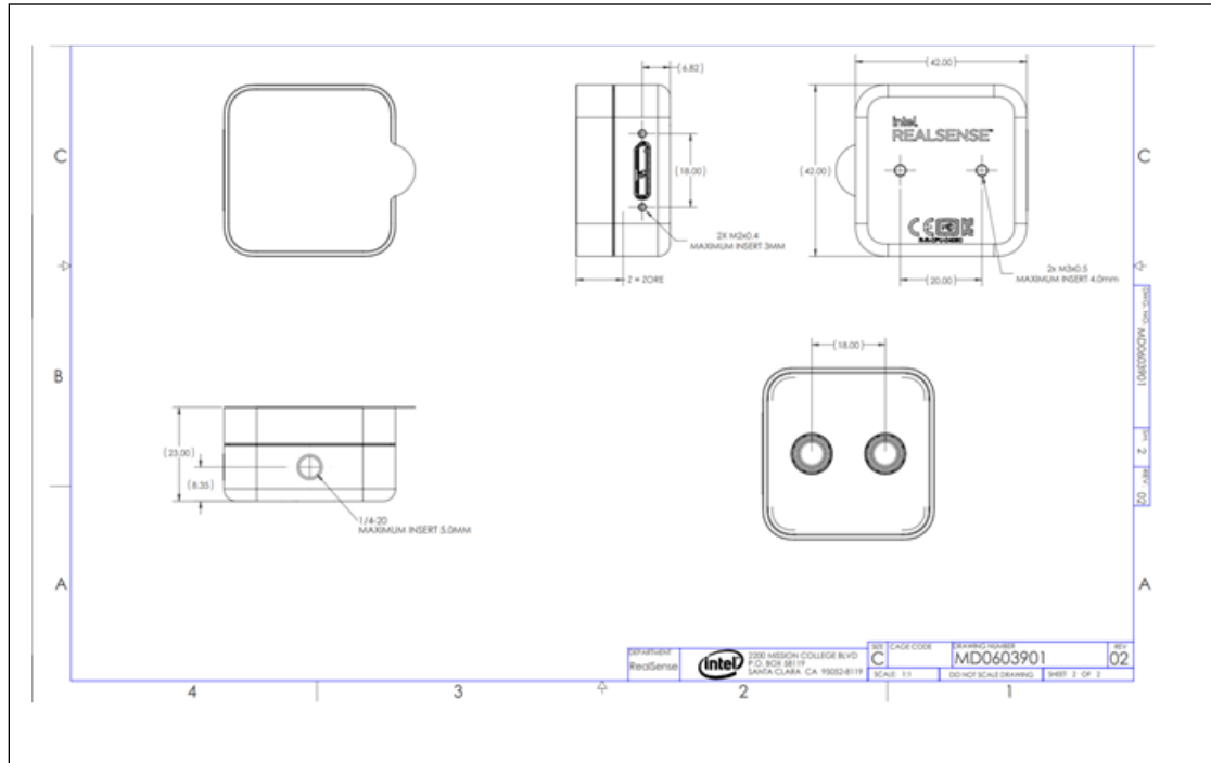
Figure 10-13. RealSense™ Depth Camera D405
