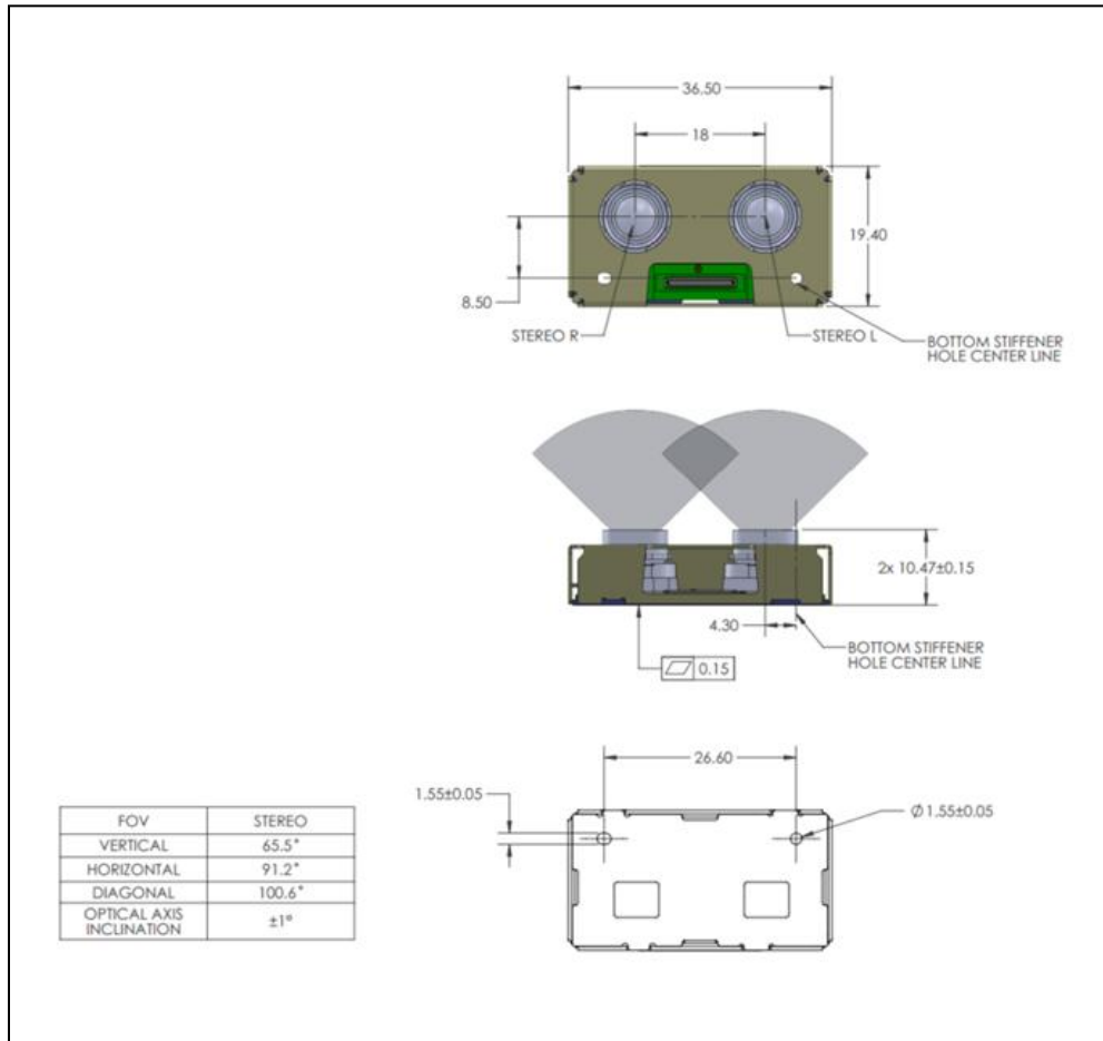
Figure 10-5. RealSense™ Depth Module D401
