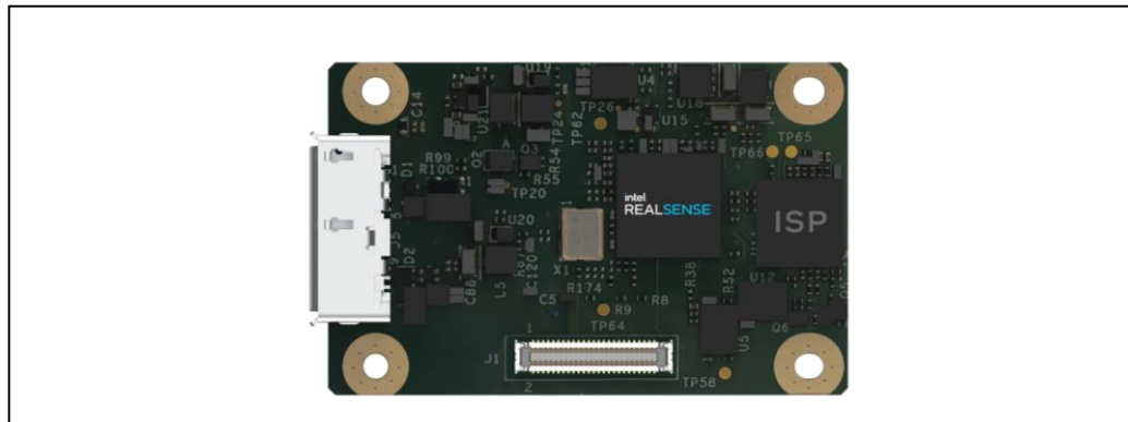
Figure 7-4. RealSense™ Vision Processor D4 Board – V4
