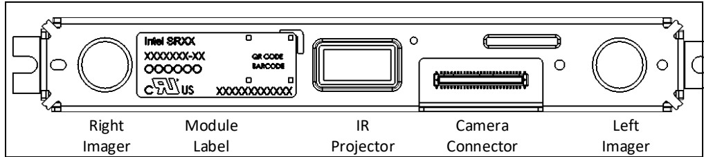
Figure 3-5. Stereo Depth Module (RealSense™ Depth Module D430)
