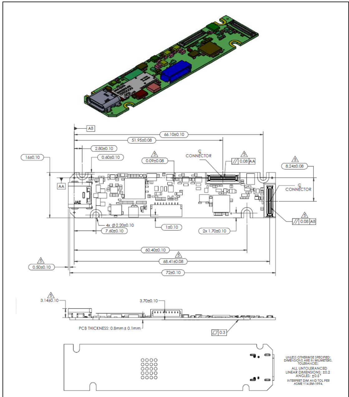
Figure 10-6. Vision Processor D4 Board USB Type-C (RealSense™ Vision Processor D4 Board – V1 and V3)
