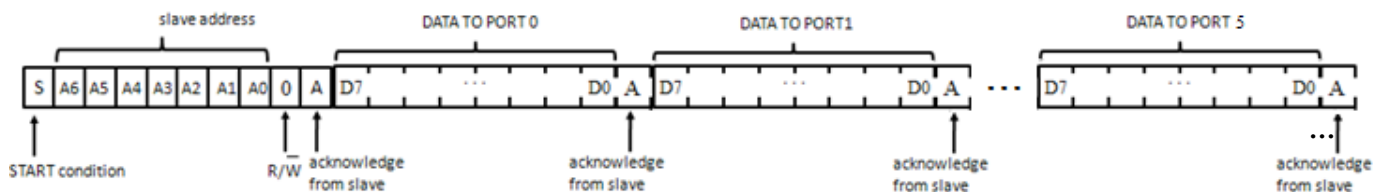
Fig 5. Write Mode
