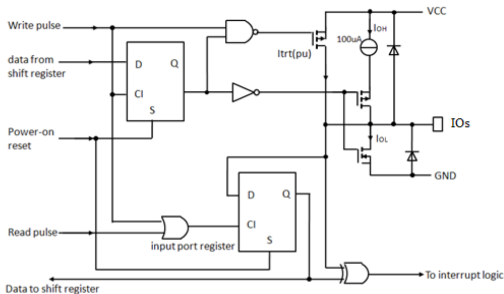
Fig 4. Simplified schematic diagram of IOX_0 to IOX_7
