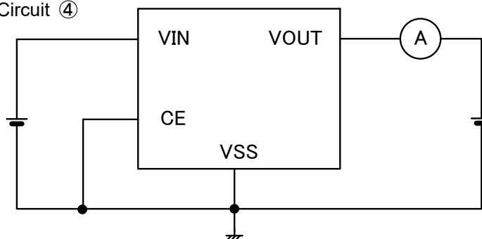
Circuit ④
