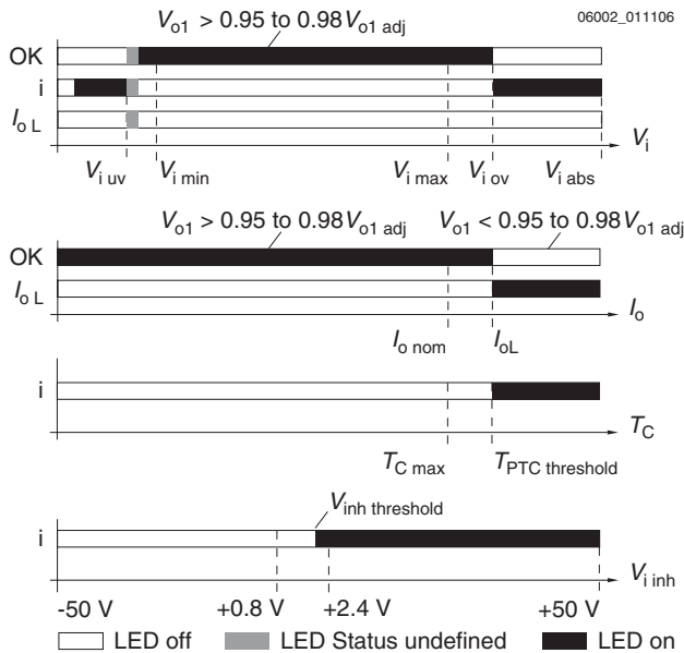
Fig. 23 LED indicators
