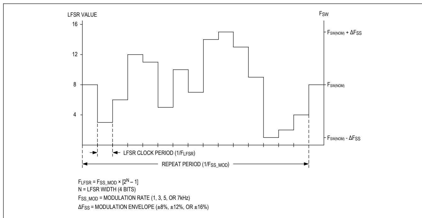
Figure 7. 4-Bit Pseudo-Random Modulation Signal Example
