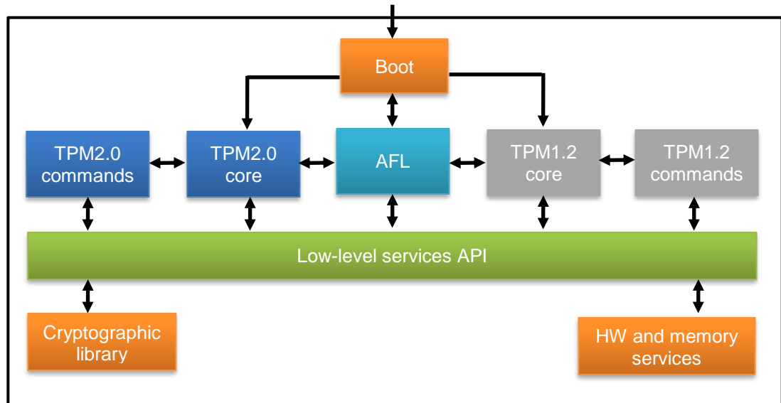
Figure 20: TPM FW block diagram (TPM2E)
