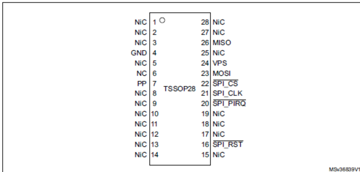
Figure 15: TSSOP28 Pinout Diagram
