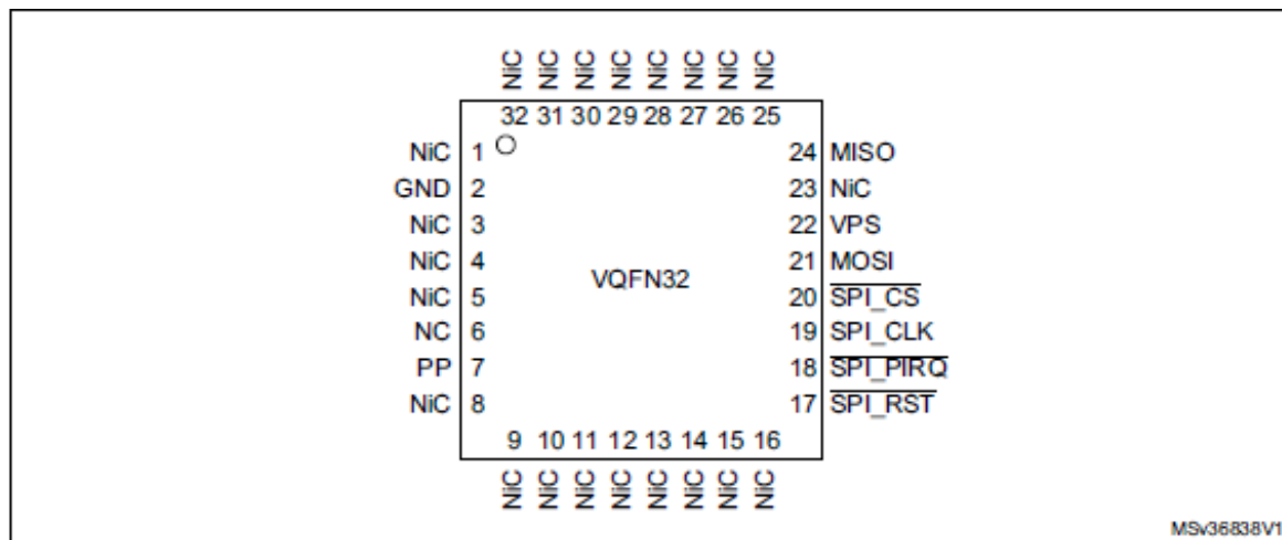
Figure 16: VQFN32 Pinout Diagram
