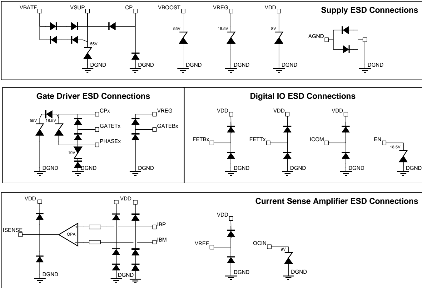
Figure 13-1 Principle Schematic highlighting ESD Connections
