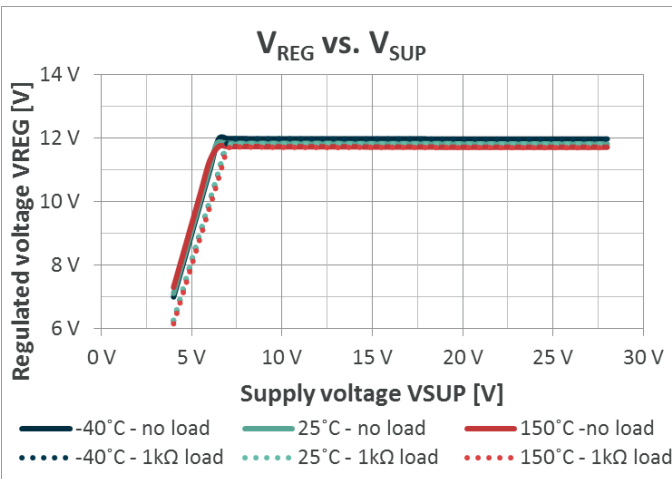
Figure 10-9 MLX83202 Regulated output voltage vs. supply voltage
