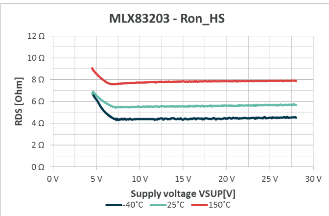
Figure 10-3 MLX83203 High-side driver FET R ON resistance vs. supply voltage
