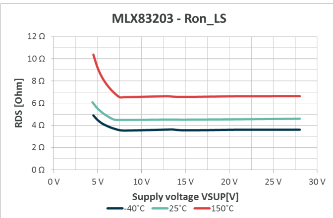
Figure 10-5 MLX83203 Low-side driver FET R ON resistance vs. supply voltage
