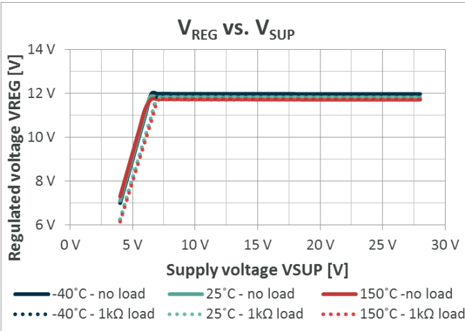
Figure 10-1 MLX83203 Regulated output voltage vs. supply voltage
