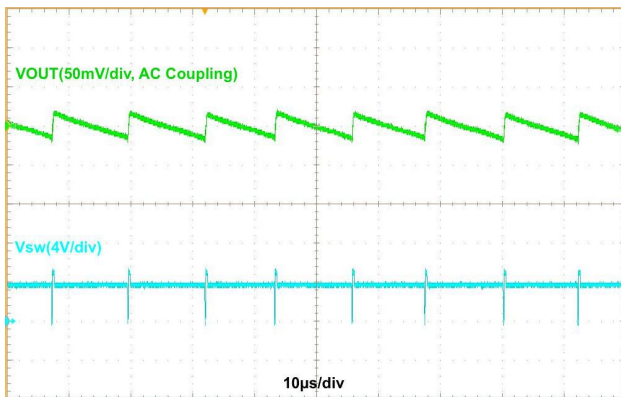
Figure 14. Boost Output Ripple in PFM Mode, V_{IN} = 3.8 V, V_{OUT} = 5.0 V, I_{OUT} = 10 mA, Auto Mode
