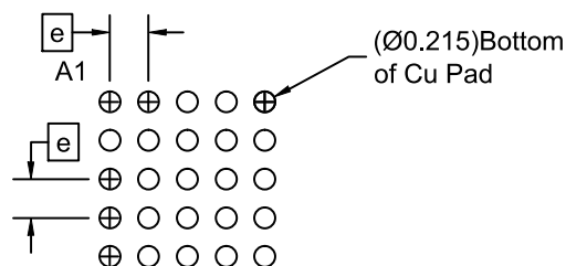
RECOMMENDED MOUNTING FOOTPRINT (NSMD PAD TYPE)
