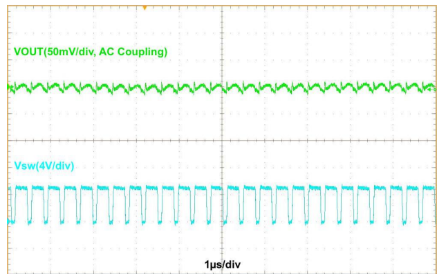
Figure 15. Boost Output Ripple in PWM Mode, V_{IN} = 3.8 V, V_{OUT} = 5.0 V, I_{OUT} = 500 mA, Auto Mode
