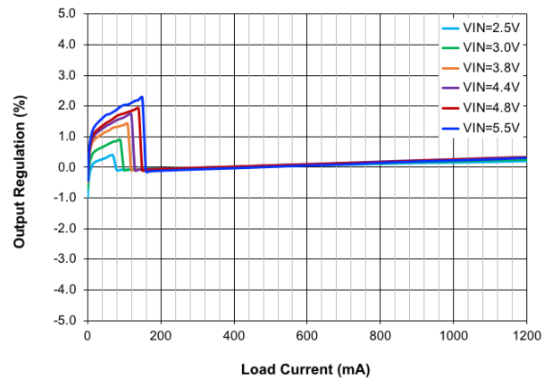
Figure 7. Buck Output Regulation vs. Load Current and Input Voltage, V_{OUT} = 1.1\text{ V} , Auto Mode
