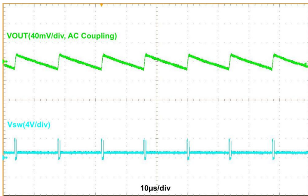
Figure 12. Buck Output Ripple in PFM Mode, V_{IN} = 3.8 V, V_{OUT} = 1.1 V, I_{OUT} = 10 mA
