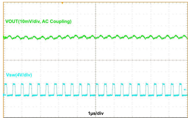
Figure 13. Buck Output Ripple in PWM Mode, V_{IN} = 3.8 V, V_{OUT} = 1.1 V, I_{OUT} = 200 mA
