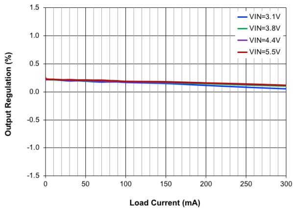
Figure 10. LDO1/2 Output Regulation vs. Load Current and Input Voltage, V_{OUT} = 2.8 V, Auto Mode
