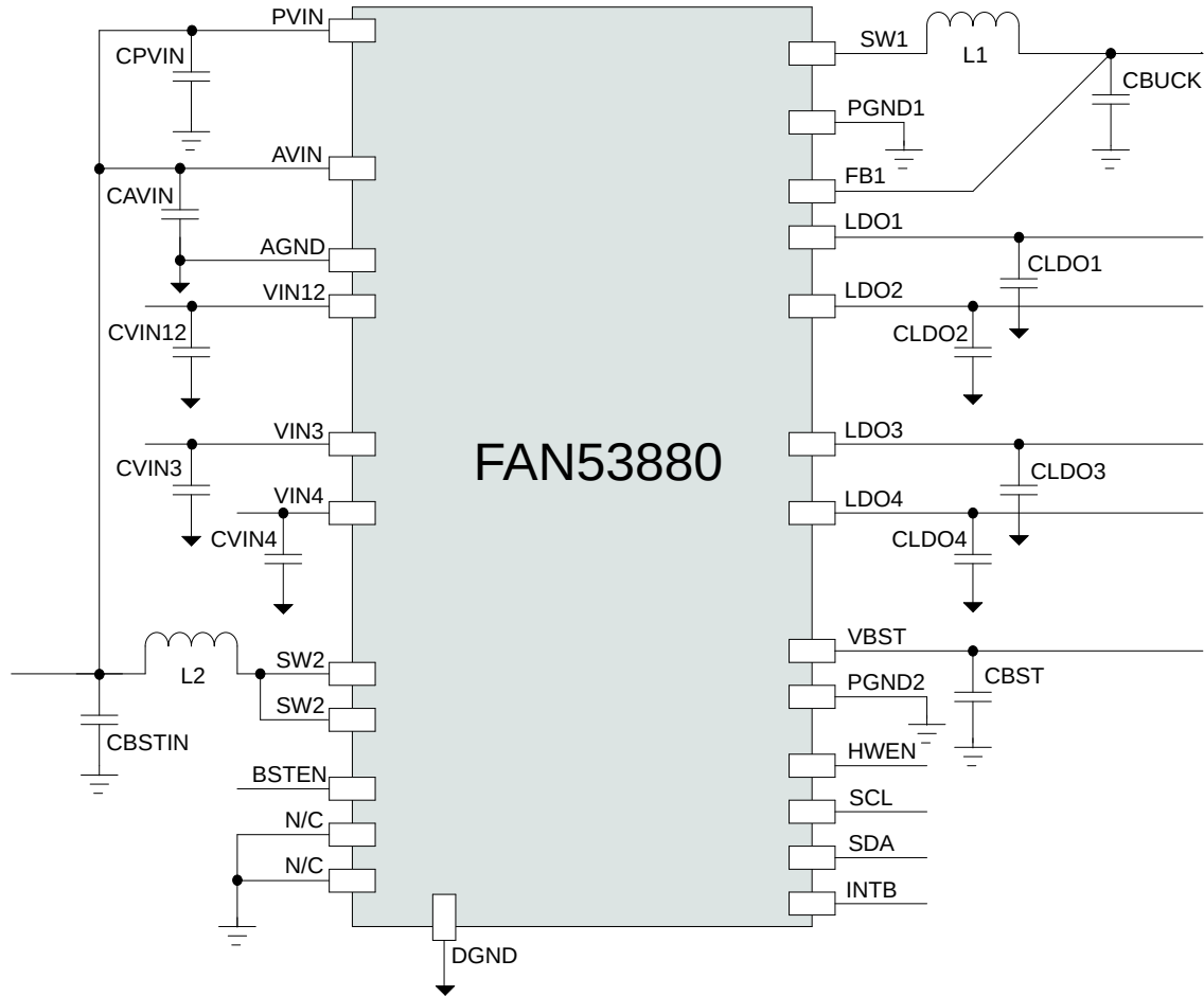
Figure 1. Application Diagram
