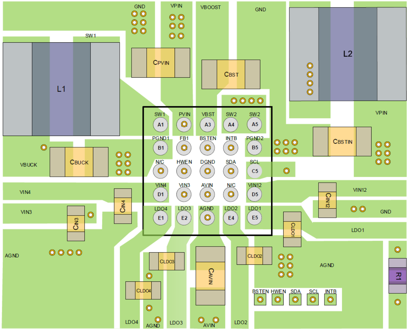
Figure 39. Layer 1
