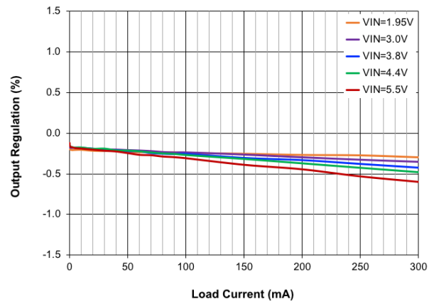
Figure 11. LDO3/4 Output Regulation vs. Load Current and Input Voltage, V_{OUT} = 1.8 V, Auto Mode
