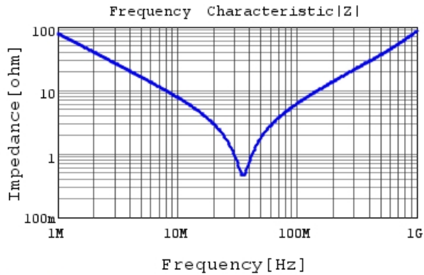
DE6E3KJ222MA3B |Z| DCOV, 20degC
