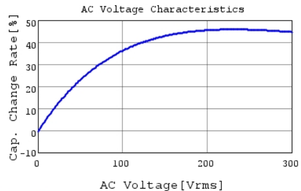
DE6E3KJ222MA3B C-AC Voltage capchange, DCOV,
