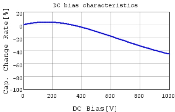
DE6E3KJ222MA3B C-DC bias capchange, 20.0degC
