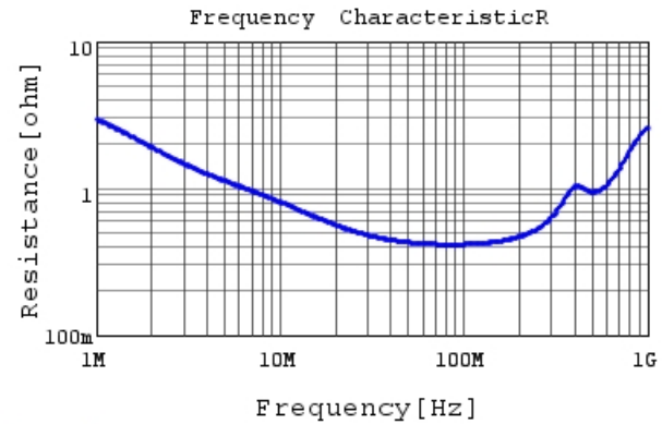
DE6E3KJ222MA3B R DCOV, 20degC
