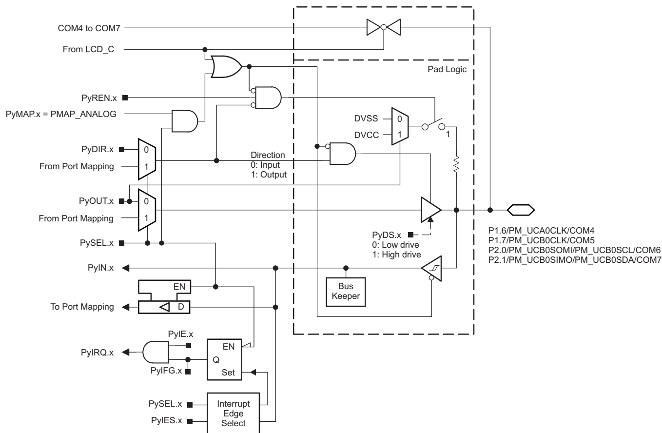
Figure 6-7. Port P1 (P1.6 and P1.7), Port P2 (P2.0 and P2.1) Diagram (PZ Package Only)
