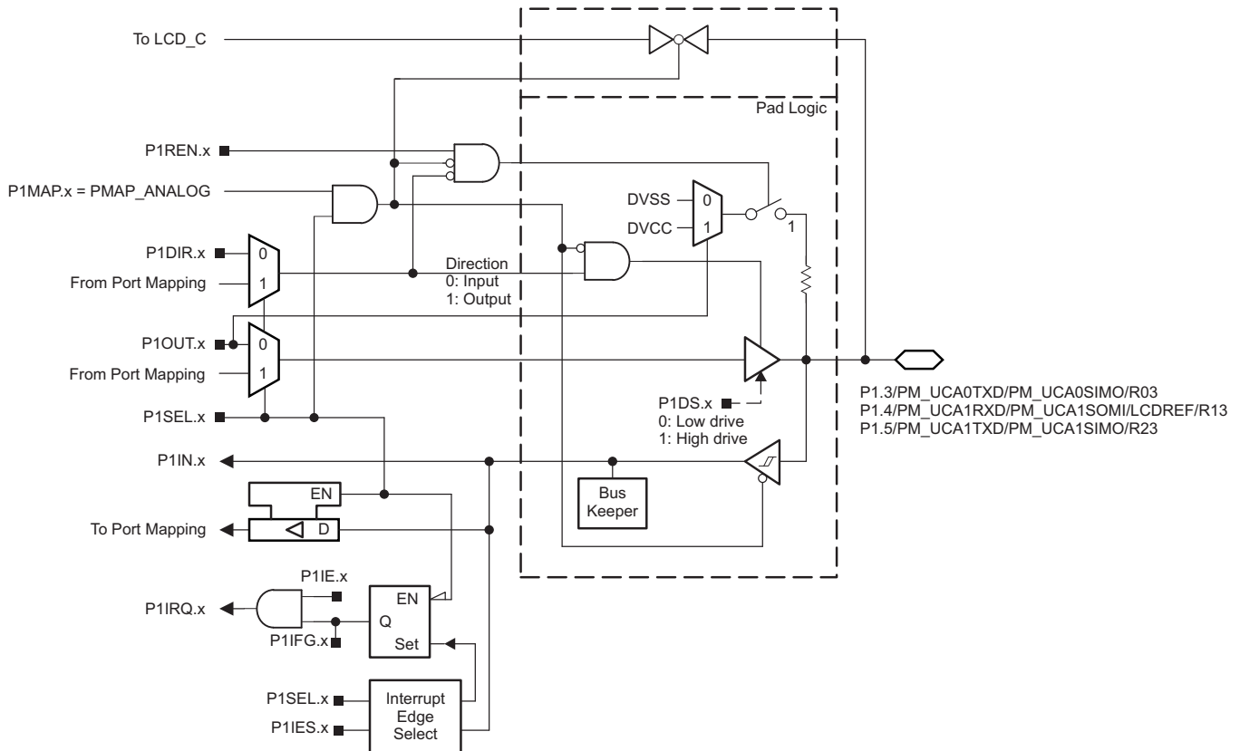
Figure 6-6. Port P1 (P1.3 to P1.5) Diagram
