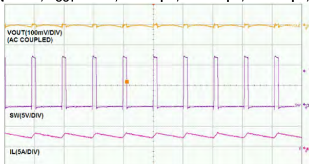
Time- 2 \mu s /div Steady State Test I_{OUT} = 3A
