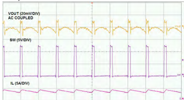
Time- 2μs/div Output Voltage Ripple
