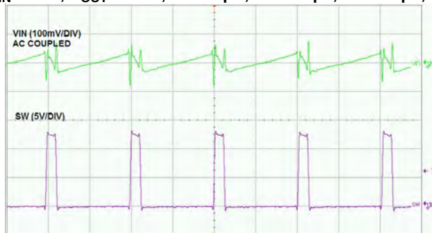
Time- 1μs/div Input Voltage Ripple
