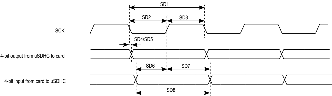
Figure 43. SDR50/SDR104 timing
