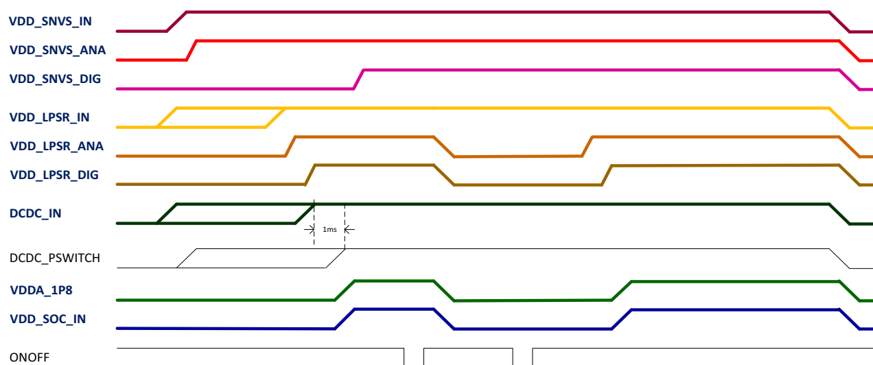
Figure 4. Power sequence
