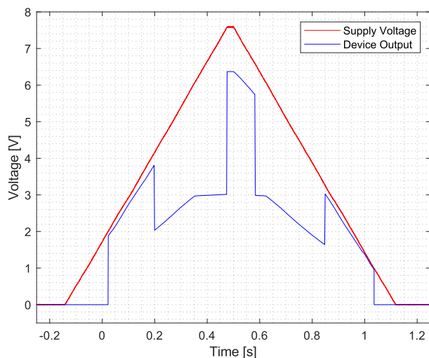
Figure 6: ACS70310 Power On/Off and OVD, no R_L
