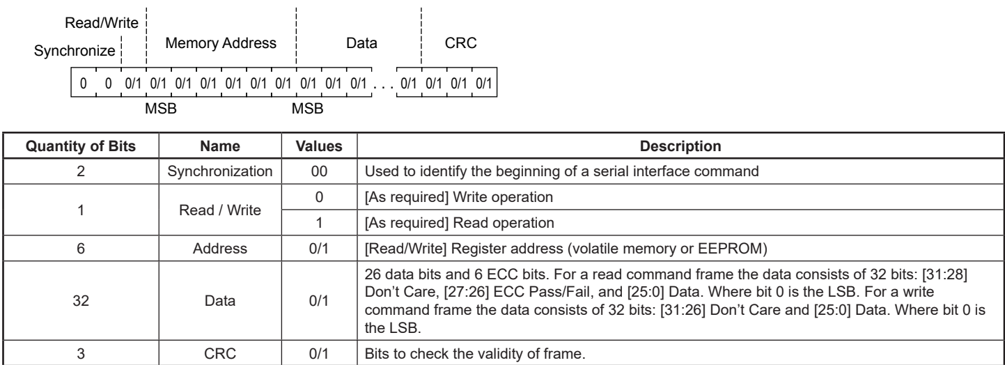
Figure 9: Command Frame General Format
