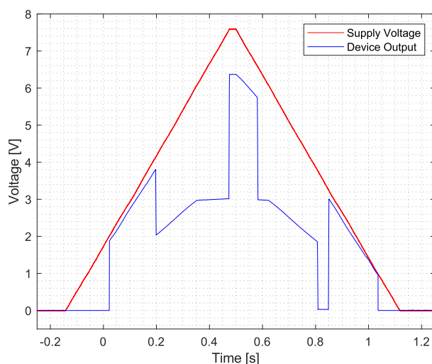
Figure 7: ACS70311 Power On/Off and UVD, R_L = 10\text{ k}\Omega
