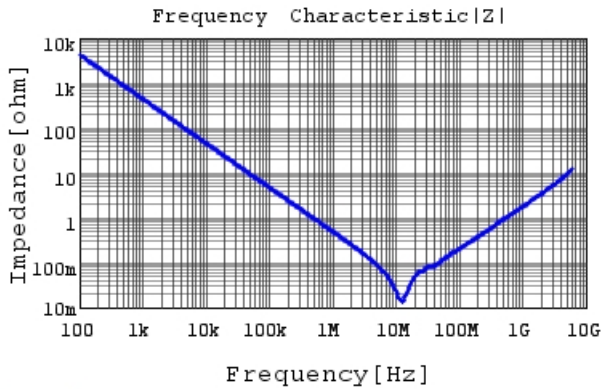
GRM188R7YA474ME05 |Z| DCOV,25degC
