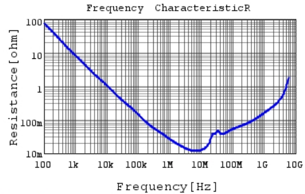
GRM188R7YA474ME05 R DCOV,25degC
