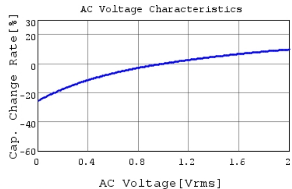
GRM188R7YA474ME05 C-AC Voltage capchange, Dc
