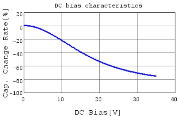
GRM188R7YA474ME05 C-DC bias capchange, 25.0C
