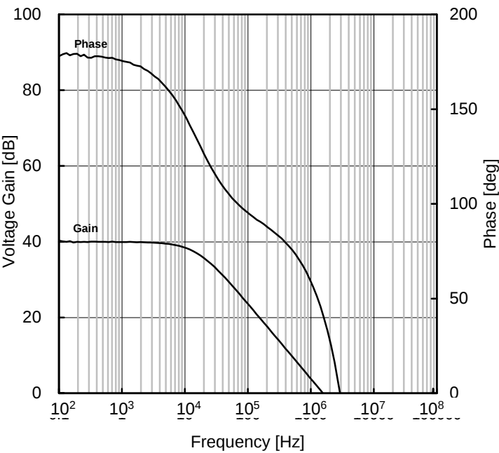
Figure 73. Voltage Gain, Phase vs Frequency
