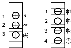
Figure 1. AC Input
