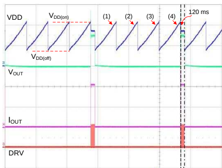
Figure 28. Soft-Short Protection
