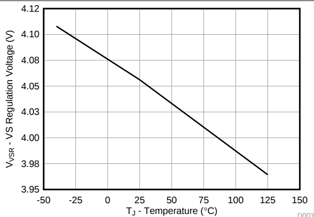
Figure 3. VS Regulation Voltage vs. Temperature
