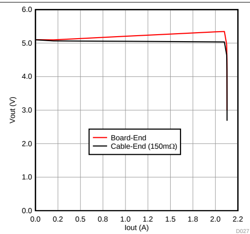
Figure 27. Output V-I Curves
