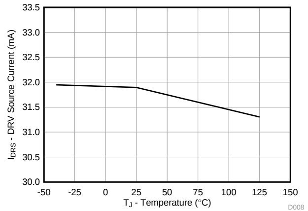
Figure 8. DRV Source Current vs. Temperature
