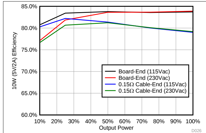
Figure 26. Efficiency
