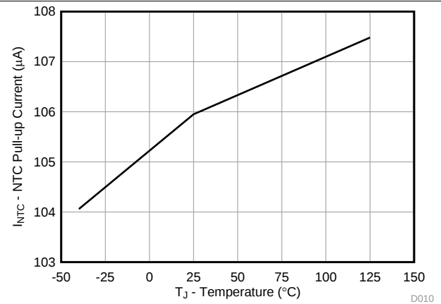
Figure 10. NTC Pullup Current vs. Temperature
