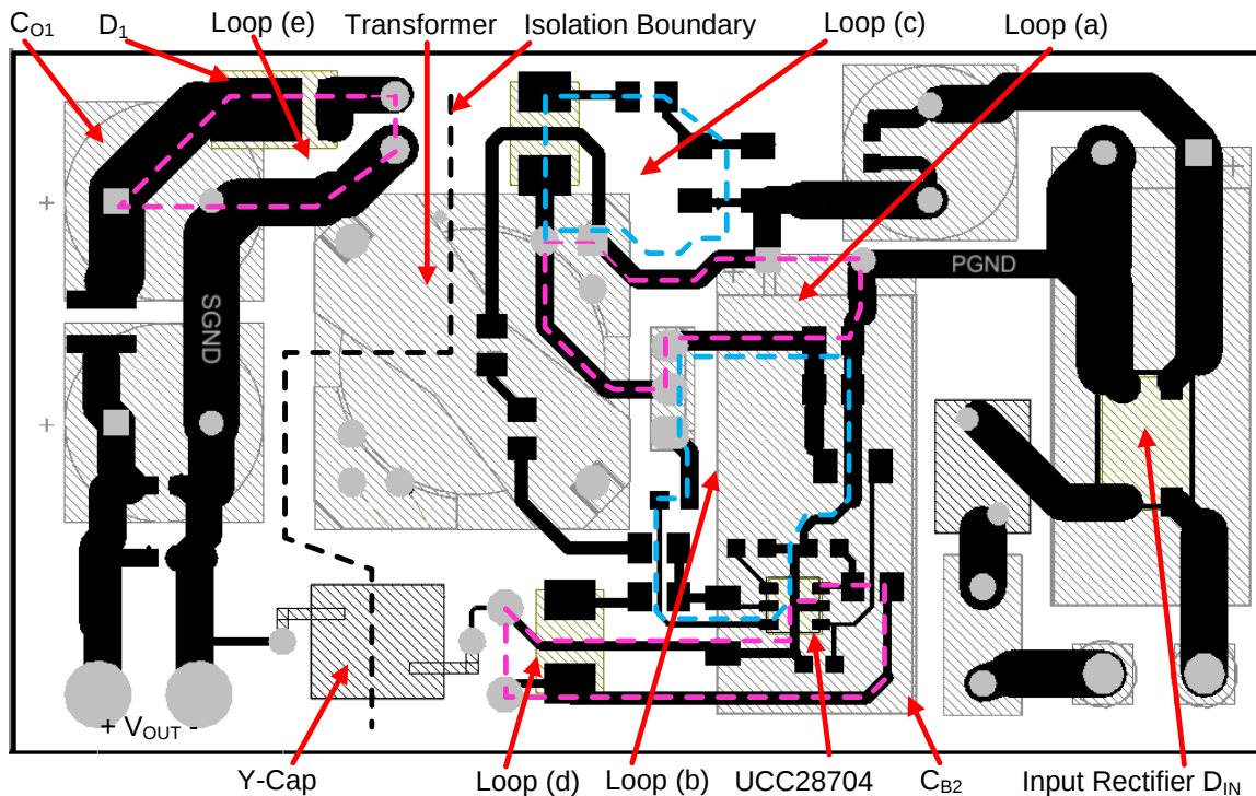
Figure 33. Layout Example
