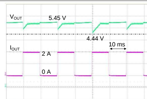
Figure 31. Typical Output Load Transient Response
