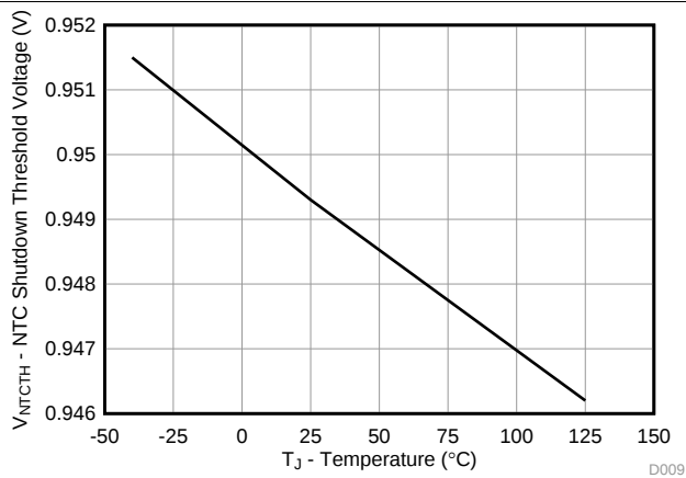
Figure 9. NTC Shutdown Threshold Voltage vs. Temperature
