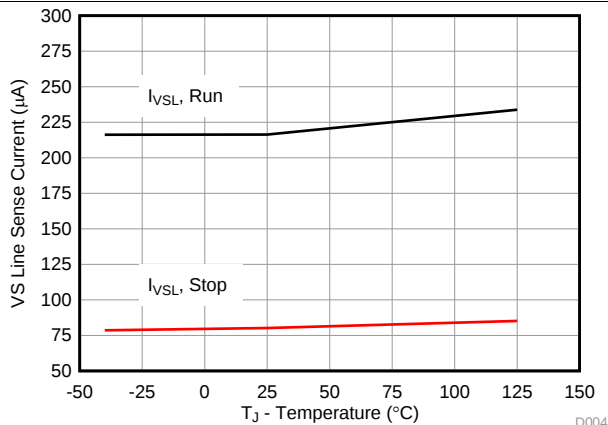
Figure 4. Line-Sense Current vs. Temperature
