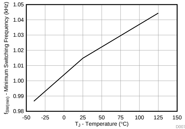
Figure 7. Minimum Switching Frequency vs. Temperature
