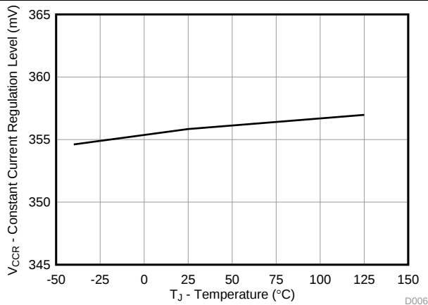
Figure 6. Constant-Current Regulation Level vs. Temperature
