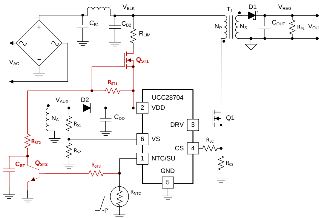
Figure 20. Power-On with a Depletion-Mode FET
