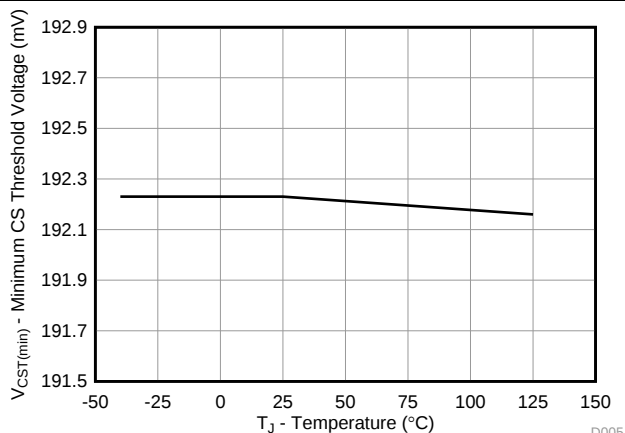
Figure 5. Minimum CS Threshold Voltage vs. Temperature
