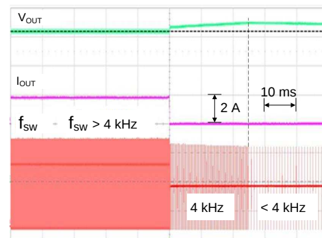
Figure 29. Response to Load Step-Down
