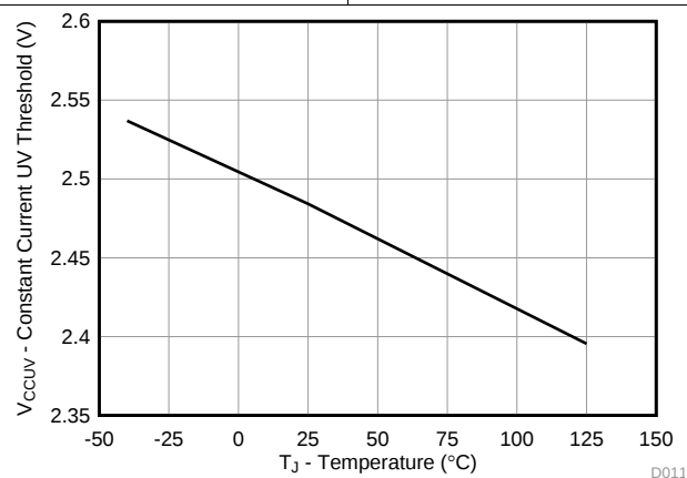
Figure 11. Constant-Current Under-Voltage Threshold vs. Temperature
