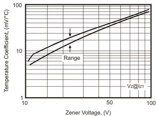
Fig.3B - Range for Units 12 to 100 Volts
