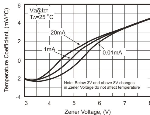
Fig.4 - Temperature Coefficients (-55°C to +150°C temperature change ; 90% of the units are in the ranges indicated.)
