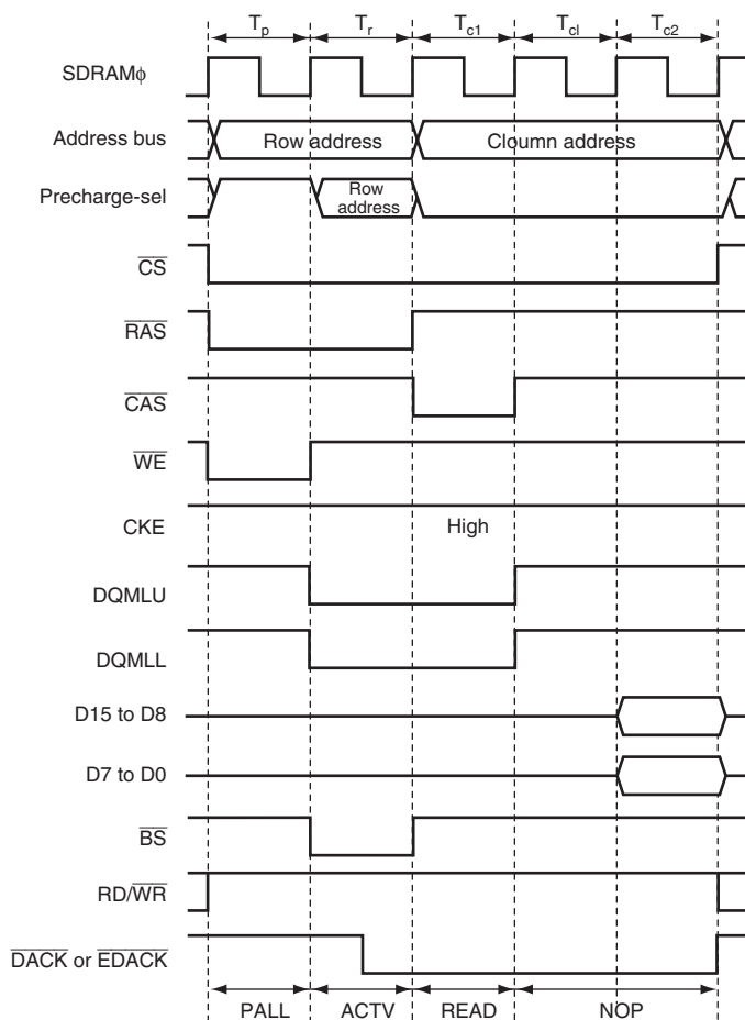
Figure 9.86 Output Timing Example of \overline{DACK} and \overline{EDACK} when DDS = 0 or EDDS = 0 (Read, CAS Latency = 2)
