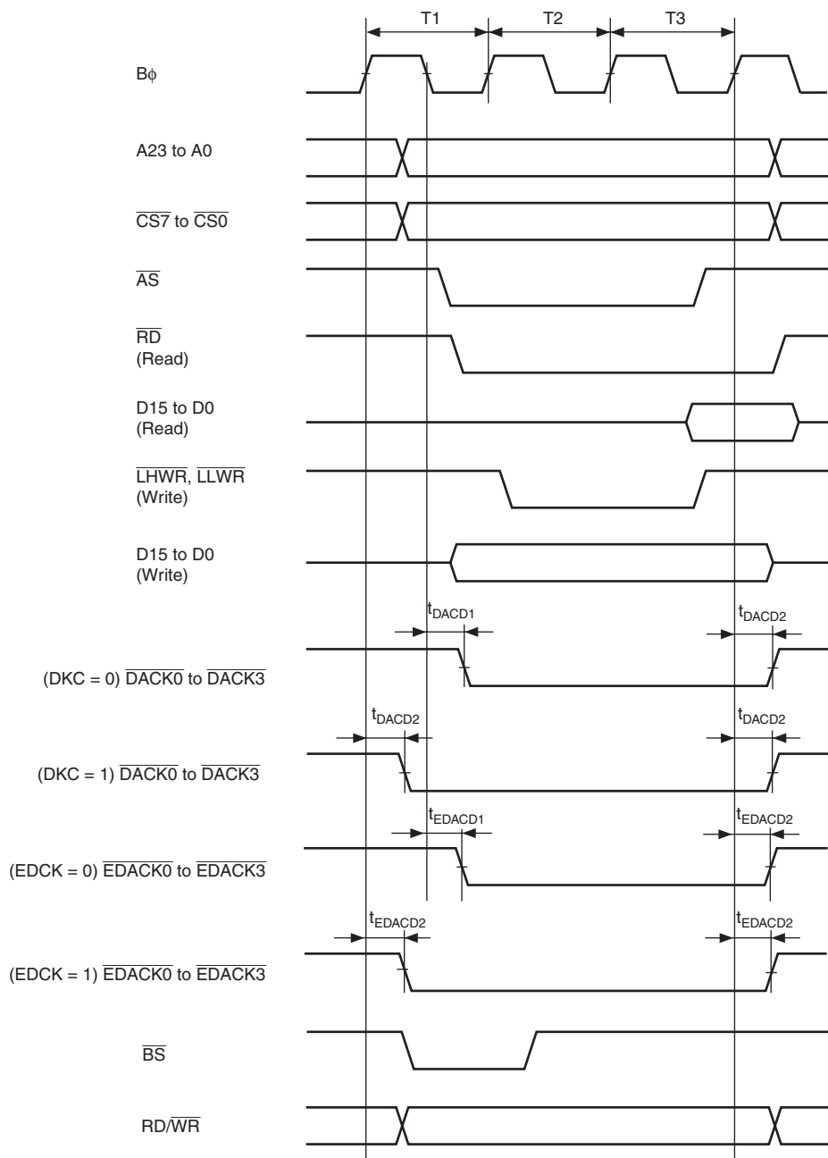
Figure 30.40 DMAC/EXDMAC Single Address Transfer Timing (3-state access)
