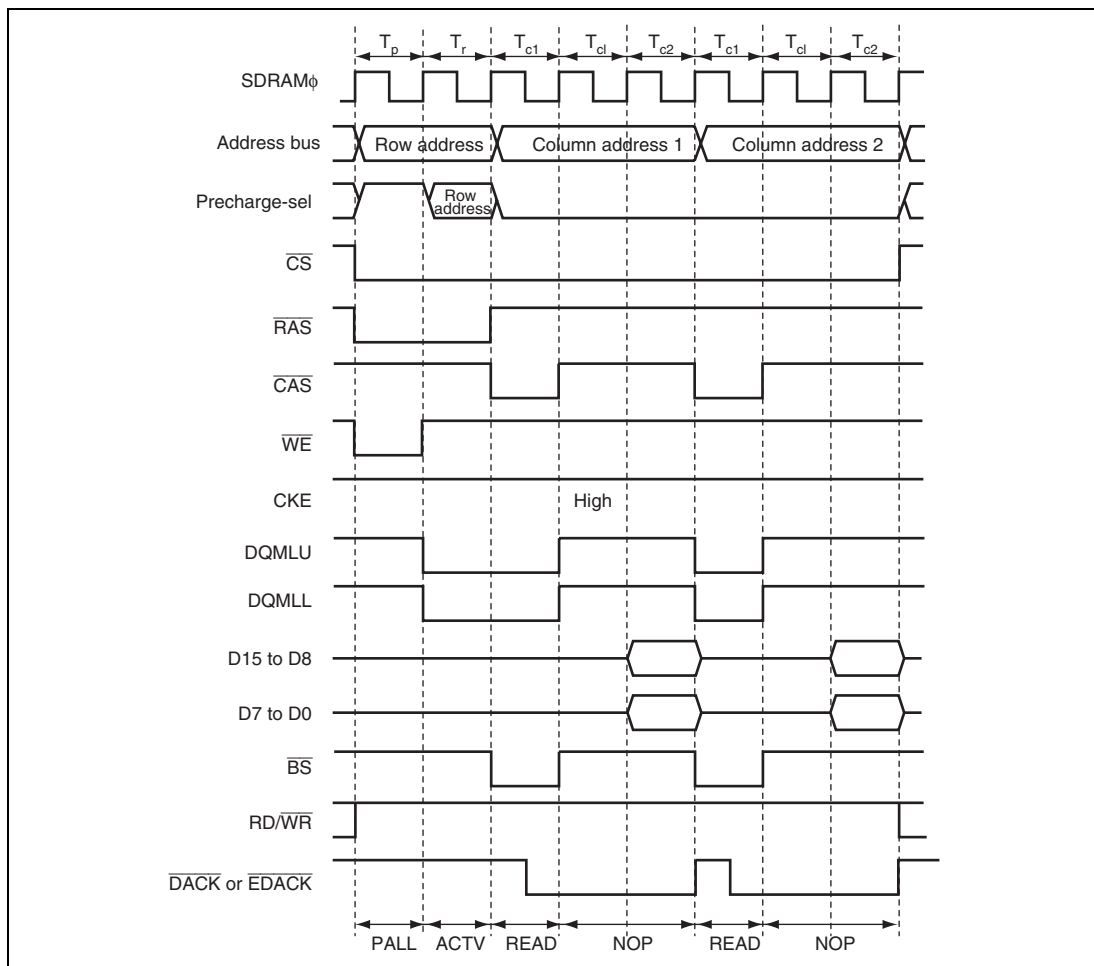
Figure 9.84 Output Timing Example of \overline{\text{DACK}} and \overline{\text{EDACK}} when \text{DDS} = 1 or \text{EDDS} = 1 (Read, CAS Latency = 2)
