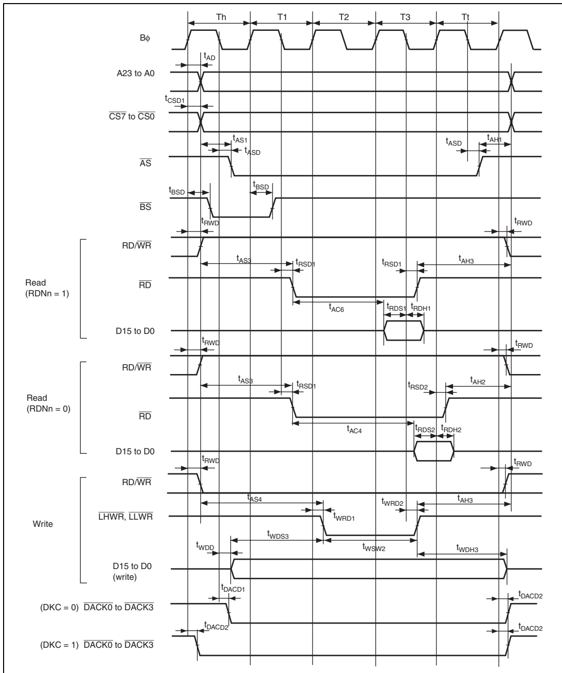
Figure 30.12 Basic Bus Timing: Three-State Access ( \overline{\text{CS}} Assertion Period Extended)
