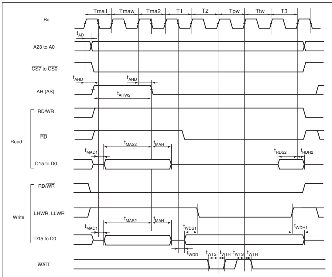
Figure 30.18 Address/Data Multiplexed Access Timing (Wait Control) (Address Cycle Program Wait \times 1 + Data Cycle Program Wait \times 1 + Data Cycle Pin Wait \times 1)
