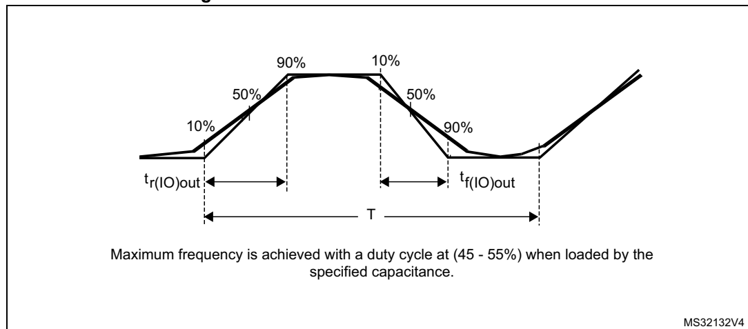
Figure 34. I/O AC characteristics definition (1)
