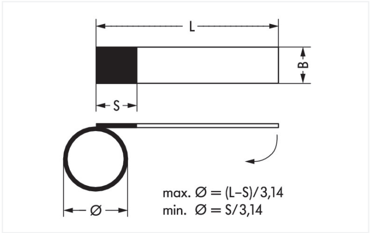
Dimensions in mm Dimensions of self-laminating label
