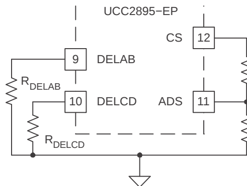
Figure 9. Resistors Needed In Programming
