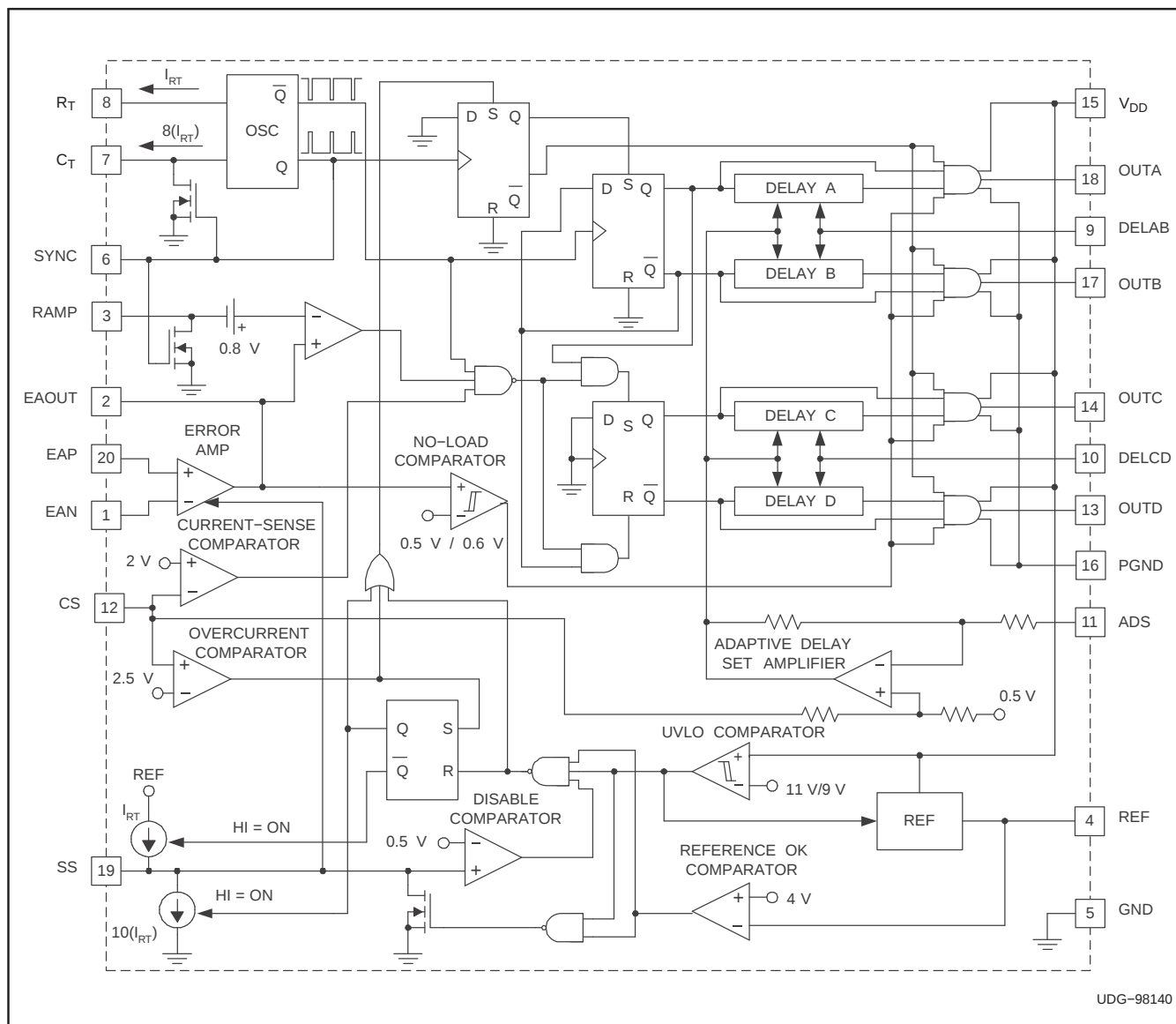
Figure 12. Block Diagram
