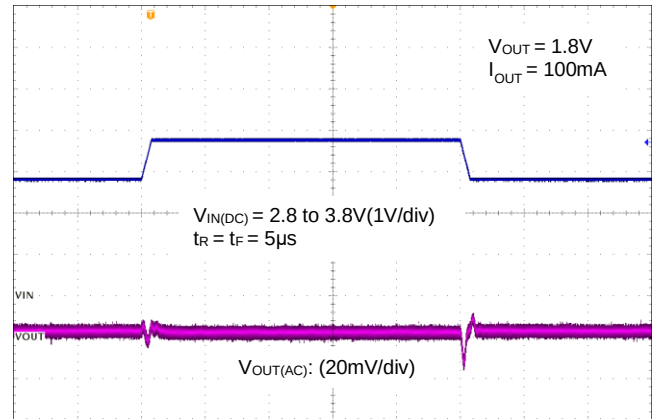
Line-Transient Response
