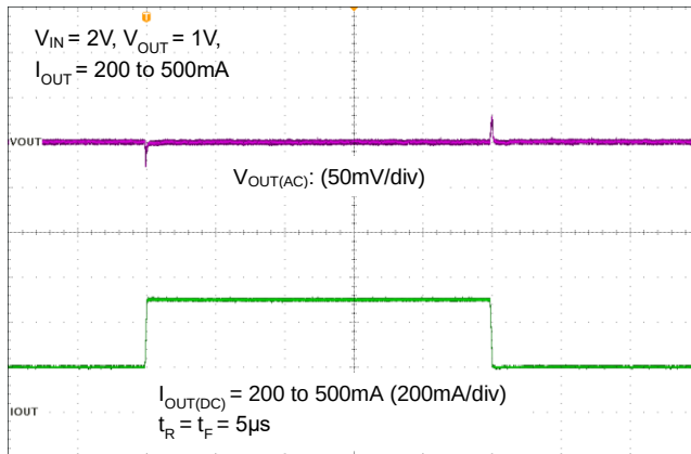
Load-Transient Response
