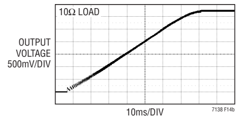
Soft-Start Waveform
