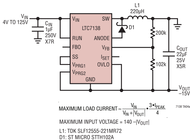
4V to 125V Input to -15V Output Positive-to-Negative Regulator
