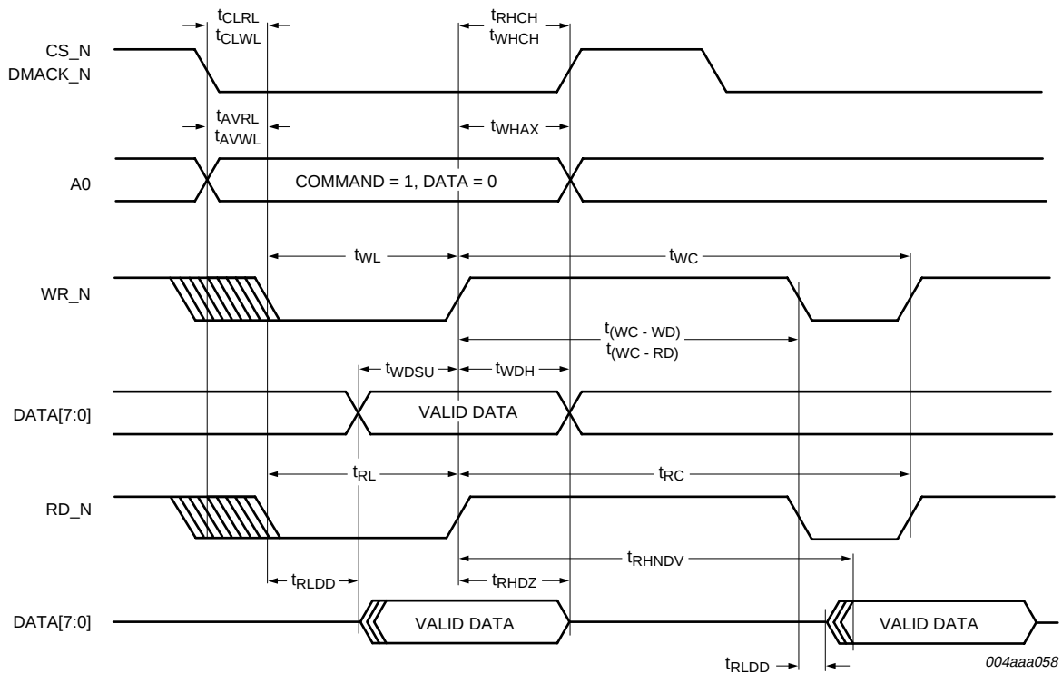
Fig 18. Parallel interface timing (I/O and DMA)
