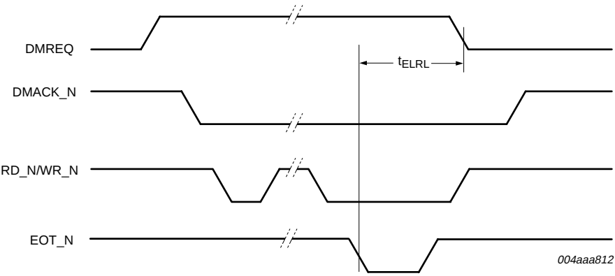
Fig 21. DMA terminated by EOT
