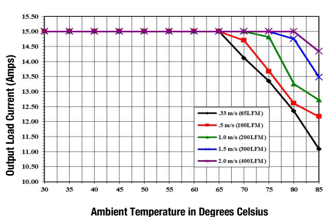
UWS-3.3/15-Q12N-C Temperature Derating Vin 24V (Airflow from Pin 1 to Pin 3 on PCB)
