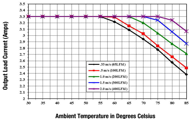
UWS-15/3-Q12N-C Temperature Derating Vin 30V (air flow from Pin 1 to Pin 3 on PCB)
