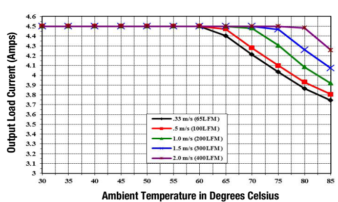
UWS-12/4.5-Q12N-C Temperature Derating Vin 12V (Airflow from Pin 1 to Pin 3 on PCB)
