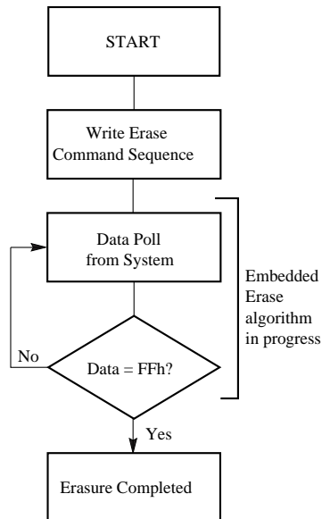
Figure 8. Erase Operation
