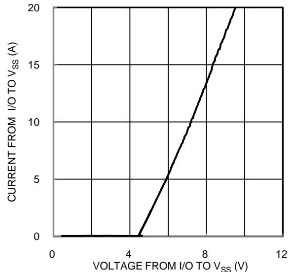
Figure 10 Current vs. Voltage
